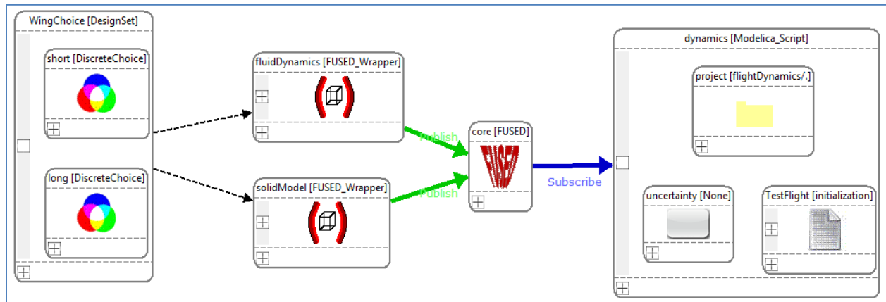
Figure 6: FUSED Composition of Solid, Aerodynamics CFD, and Vehicle Dynamics Models
