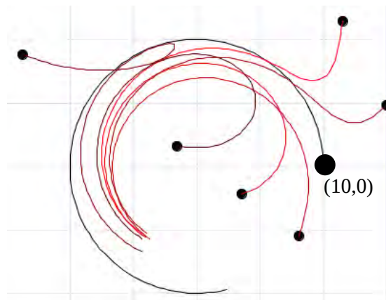
Figure 1: Pursuit paths for several pursuers chasing an evader’s circular path.
