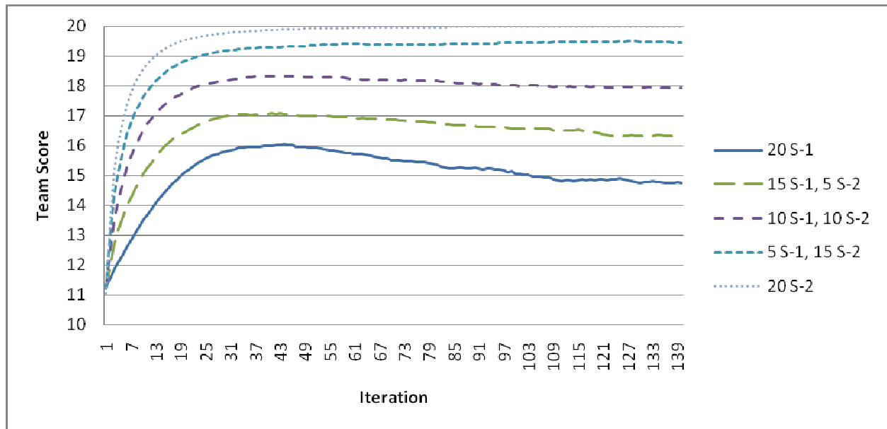
Figure 4: Teams scores reflecting average closeness to equi-distribution for five teams of 20 players each with various compositions of players using the S-1 and S-2 algorithms (as indicated in the margin). Each line represents the average of 200 runs for different sets of initial conditions, with each run consisting of 140 iterations.
