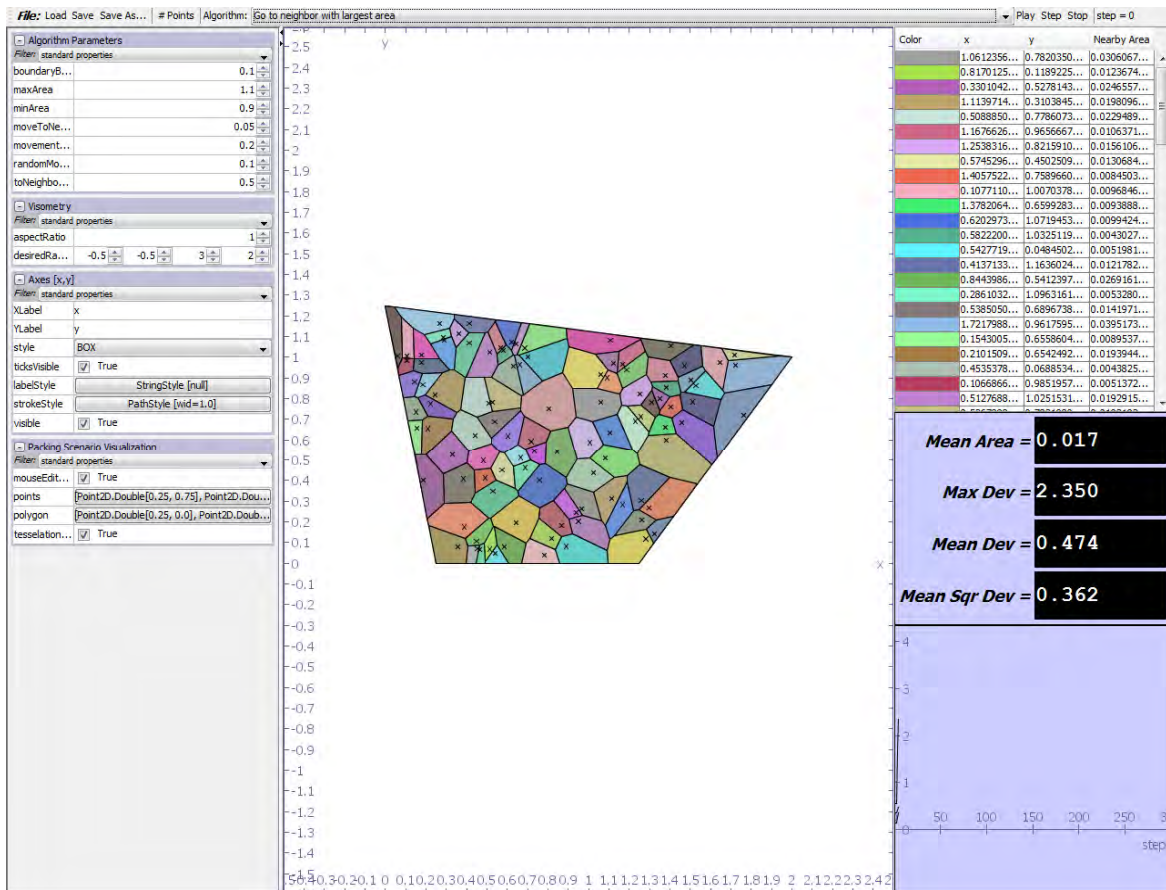
Figure 2: JAVA-based simulation platform for geometric distribution algorithms
