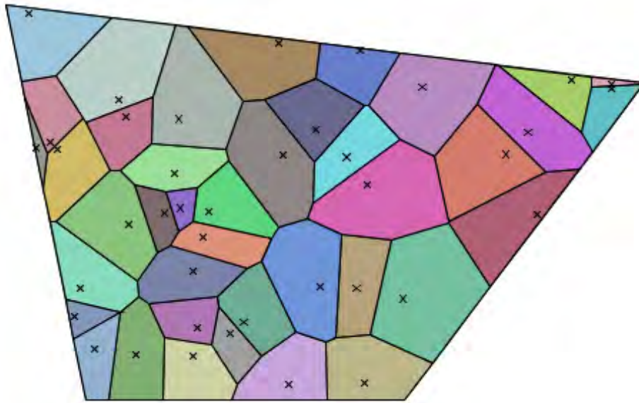
Figure 1: Initial “meshed” region with 40 points (unequal areas). This region has poor utility metrics --- e.g., the maximum assigned area for the largest entity is 140% of the mean area.
