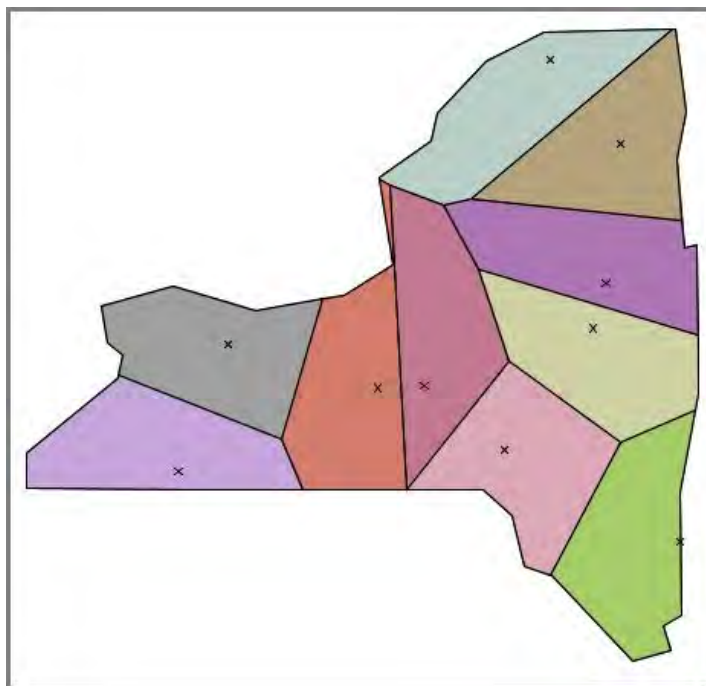
Figure 6: Result of the S-2 algorithm distributing 10 satellites over New York State.
