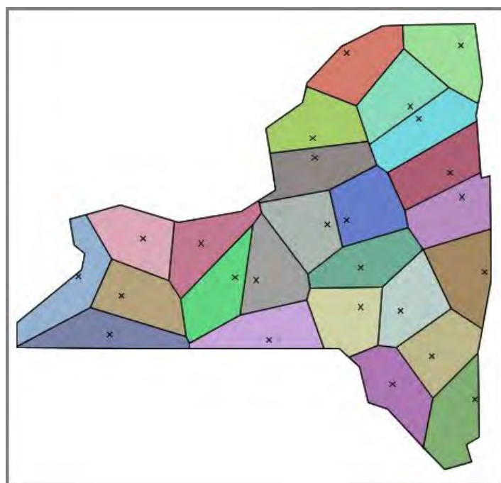
Figure 7: Result of the S-2 algorithm distributing 25 satellites over New York State.
