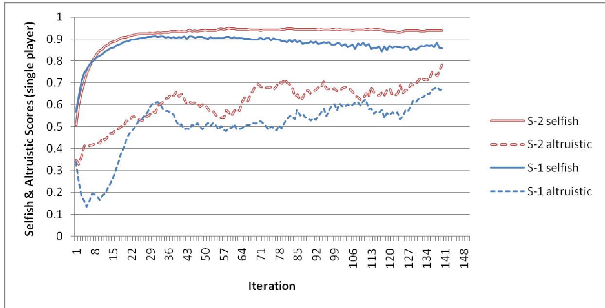
Figure 5: Selfish and altruistic scores for players operating with S-1 and S-2 algorithms on a team with 10 S-1 players and 10 S-2 players. Each line represents the average of 200 runs for different sets of initial conditions, with each run consisting of 140 iterations. Despite some noise in the results, there is clear evidence that the S-2 algorithm is more altruistic.
