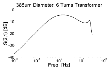
Figure 37 S_{21} for a 385 \mu m transformer
