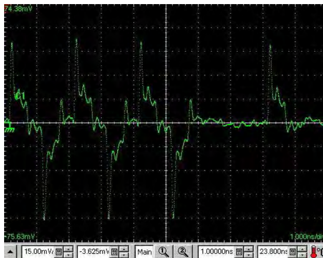
Figure 66 Channel output for full swing input for the transition bit only at 1 Gbps; power is 17 mA
