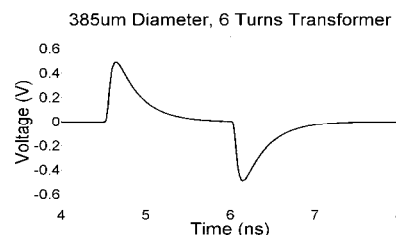
Figure 38 Output from a 385 \mu m transformer
