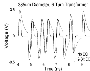
Figure 44 Output from a 6-turn transformer with and without fractionally equalized input at 4 Gbps
