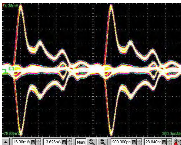
Figure 67 Eye diagram for channel output using an NRZ input signal at 1 Gbps
