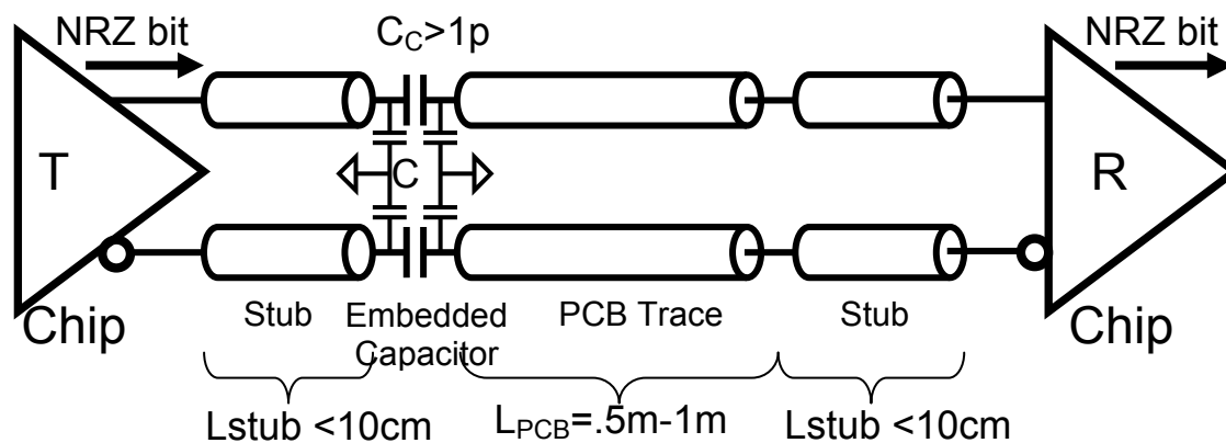
Figure 30 Simplified model of ACCI channel
