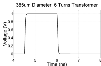
Figure 36 NRZ input for a 385 \mu m transformer
