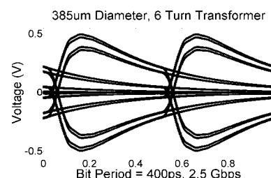
Figure 41 Eye diagram illustrating ISI due to the natural decay of the pulse tail
