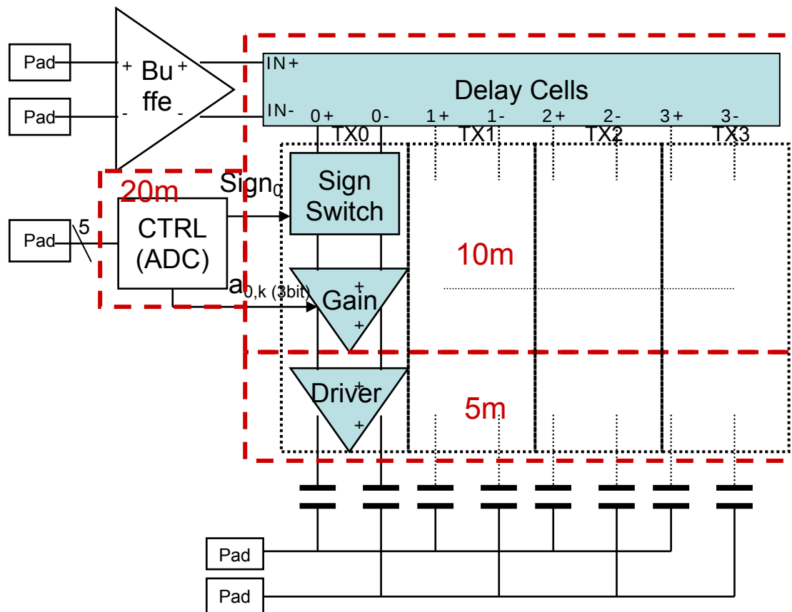
Figure 13 Transmitter circuit
