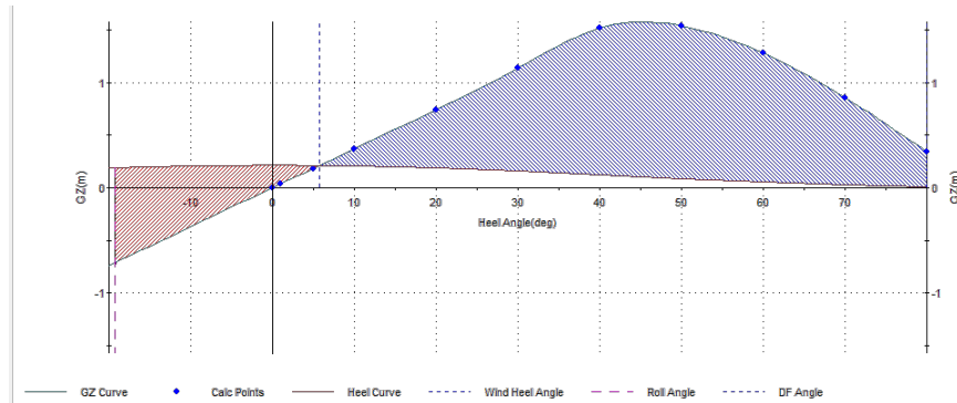
Figure 36 - Full Load GZ Curve
