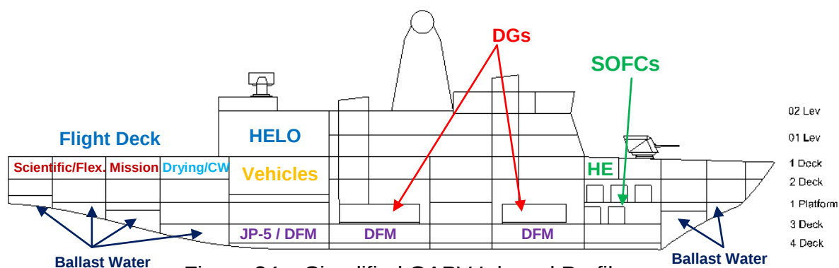
Figure 24 – Simplified GAPV Inboard Profile
