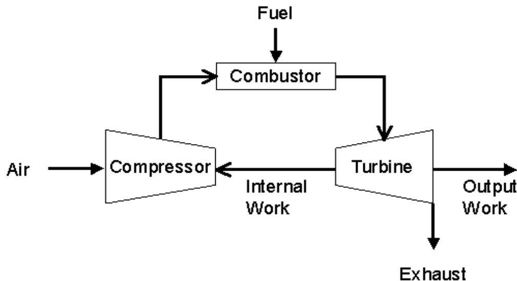
Figure 5: Brayton cycle
