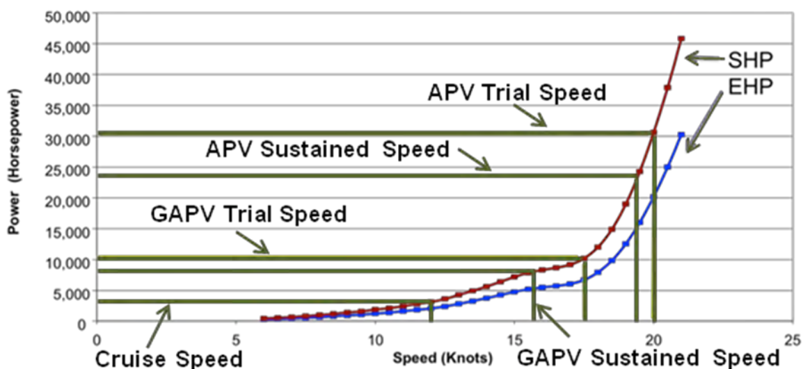
Figure 2: Powering requirements
