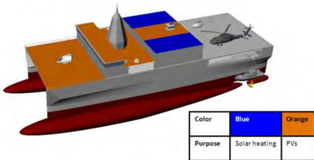
Proposed location of PVs and solar heating tubes for GAPV
