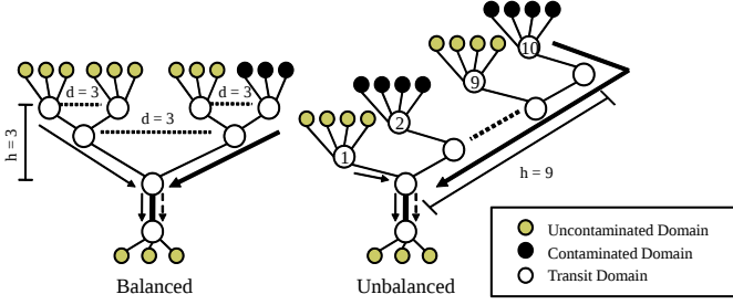
Fig. 3: Topology used in simulation.
