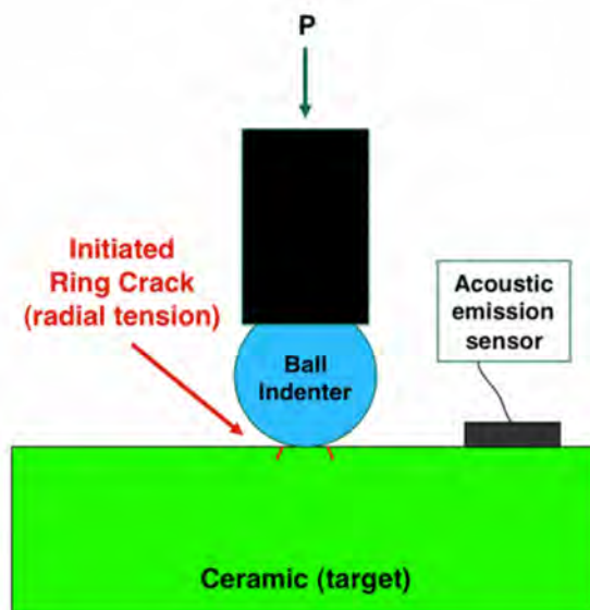
Figure 1. Schematic drawing of the ring crack initiation test configuration. An acoustic emission sensor was used to detect an acoustic event that was then linked to the ring crack initiation force. Target material is Starphire SLS glass.
