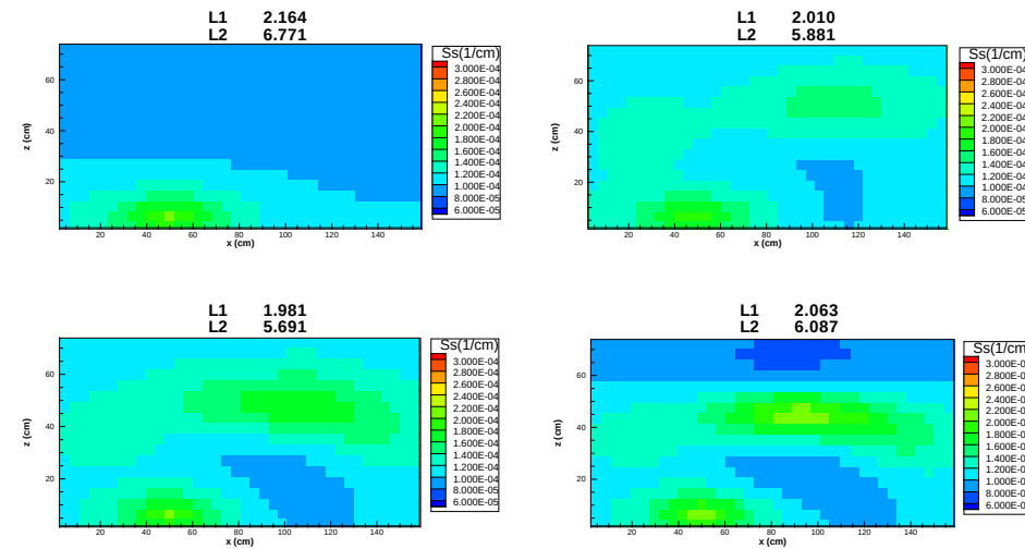
Figure 11.5: S_s tomograms computed using HT-m from synthetic pumping test data included sequentially. a) Ports 47, 44. b) Ports 47, 44, 35, 32. c) Ports 47, 44, 35, 32, 17, 14. and d) Ports 47, 44, 35, 32, 17, 14, 5, 2. Port numbers indicate the ports used as the pumped well for each cross-hole test.
