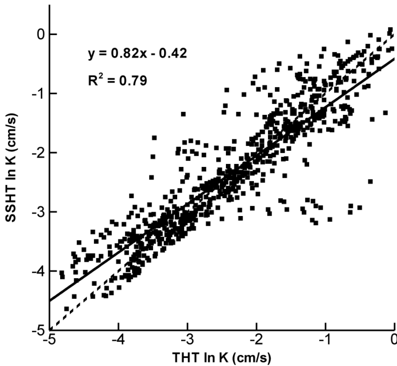
Figure 13.6: Scatterplot of ln- K from transient hydraulic tomography [this paper] to ln- K obtained using steady state hydraulic tomography [ Illman et al. , 2010]. The dashed line is a 1:1 line indicating a perfect match. The solid line is a best fit line, and the parameters describing this line are only each plot.
