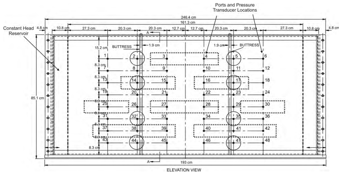
Figure 8.1: Computer Aided Design [CAD] drawing of sandbox used for the validation of hydraulic tomography. Low K blocks are shown as dotted lines and circles around the numbers indicate the ports used for pumping.
