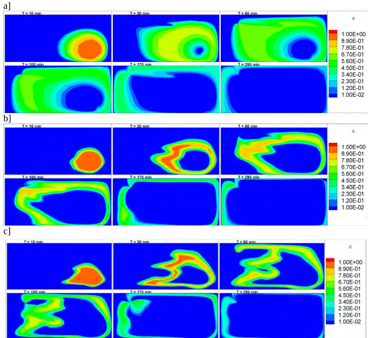
Figure 16.8: Concentration distributions from tracer transport simulation with: a) K_{eff} and A_{11} computed using Gelhar and Axness [1983] solution with statistics of permeameter analysis of core samples [case 1]; b) kriged K field [case 2]; and c) K tomogram [case 3].
