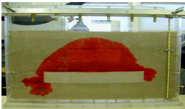
Figure 15.2: Photograph of the TCE source zone after TCE migration has stopped.
