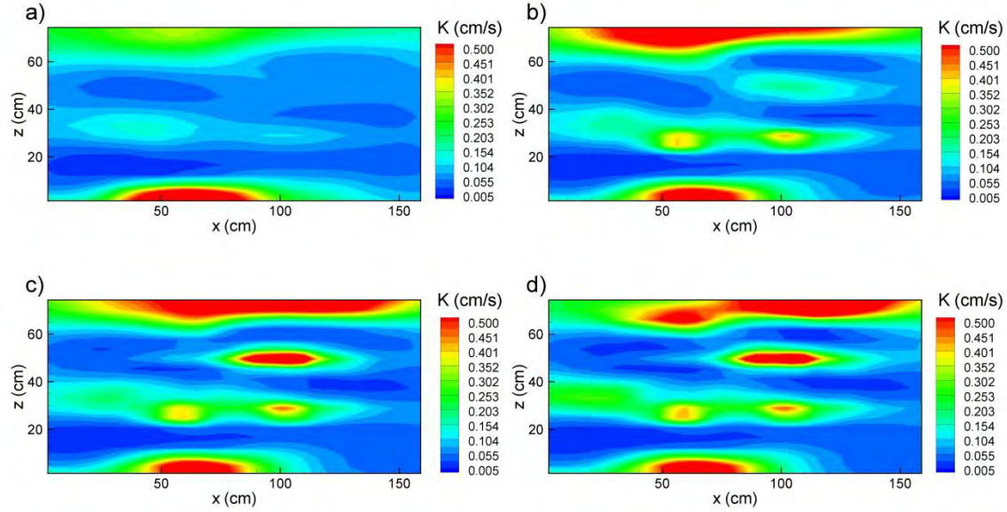
Figure 12.5: K tomograms computed using: a) 2 pumping tests [ports 47 and 44]; b) 4 pumping tests [ports 47, 44, 35, and 32]; c) 6 pumping tests [ports 47, 44, 35, 32, 17, and 14]; and d) 8 pumping tests [ports 47, 44, 35, 32, 17, 14, 5 and 2].
