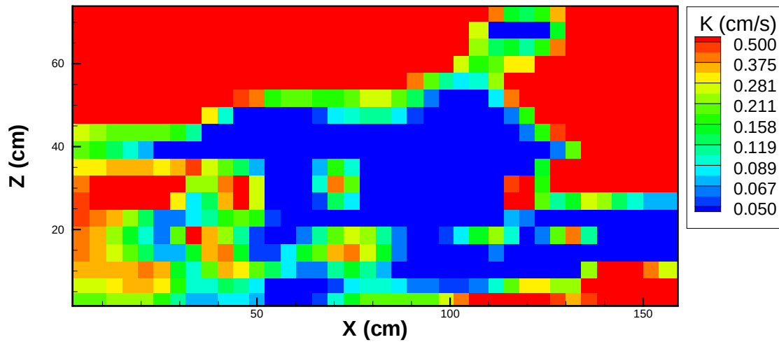
Figure 9.3: K tomograms obtained from low Q pumping test data with lower signal-to-noise ratio for the: a] synthetic and b] real cases.
