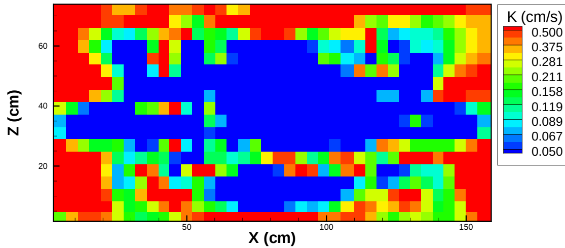
Figure 9.4: K tomograms obtained by varying the order of pumping test data included in the SSLE algorithm for the: a] synthetic and b] real cases.
