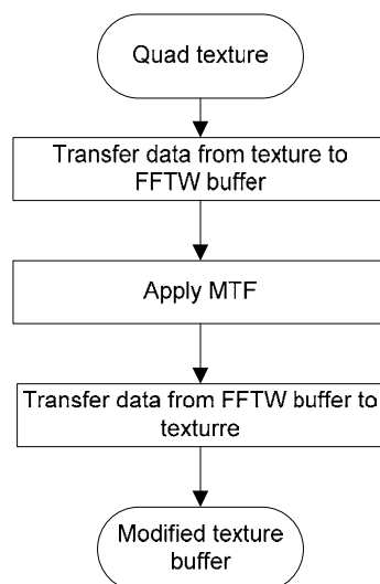
Figure 51: General process to apply MTF on the texture.
