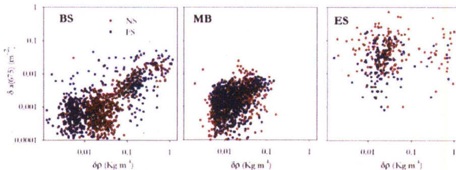
Fig. 3 Biological versus physical mechanisms modulating vertical distribution of optical properties. Vertical variation ( \delta ) of a(675) and seawater density ( \rho ) per meter is plotted in log10 scale. Each data point corresponds to the arithmetic average within 1 m bin. Ascending and descending Scanfish measurements are included.
