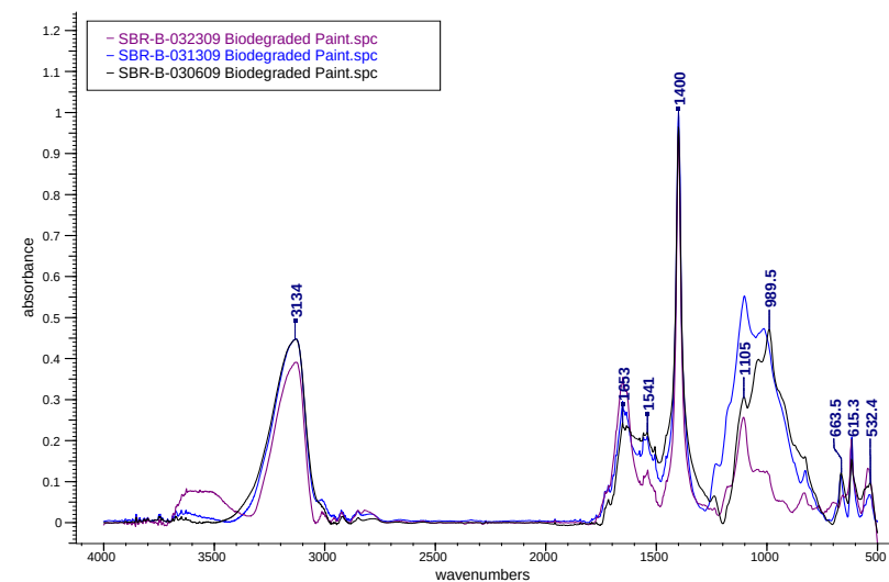
Figure 6-26. FTIR spectra of biodegraded epoxy polyamide resin.
