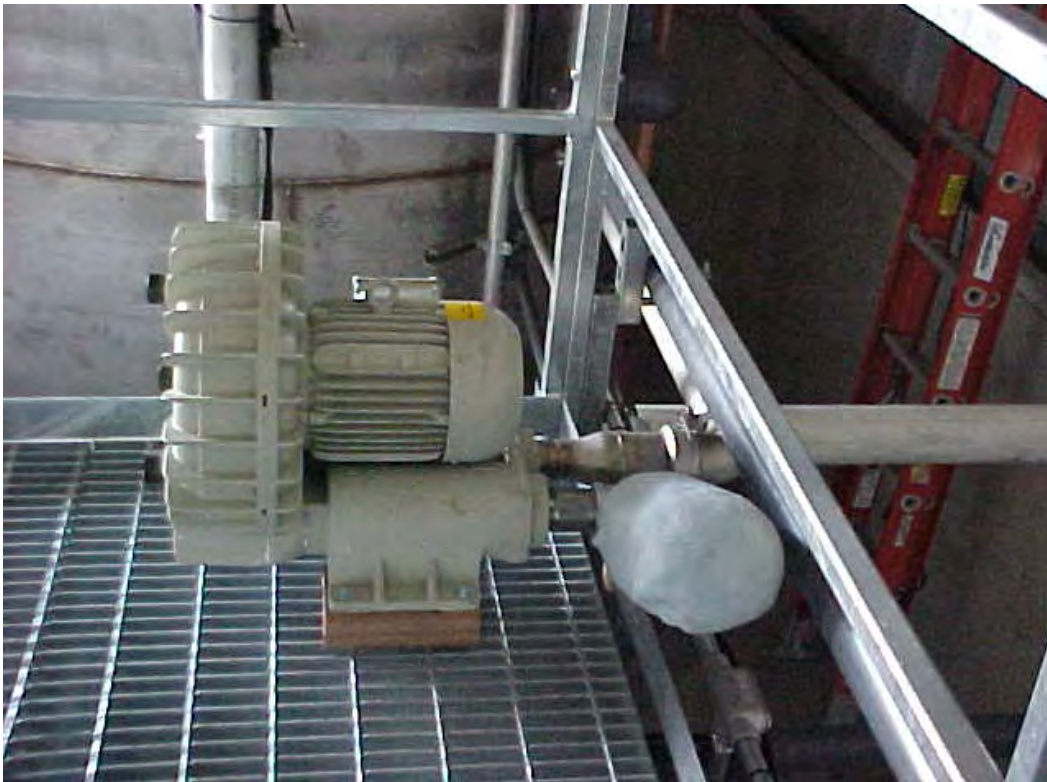
Figure 5-8. Blower.
