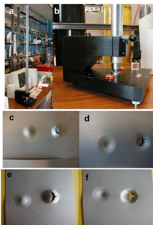
Figure 5-31 Photographs of the ASTM D-2794-93 impact setup from Gardner (a and b), impacted area of the 2 um thick ZSM-coated AA-2024 panel (c and d for each side, and left mark for impact from 1 ft and right mark for impact from 2 ft) and impacted area of the 7.5 um thick ZSM-coated AA-2024 panel (e and f for each side, and left mark for impact from 1 ft and right mark for impact from 2 ft)
