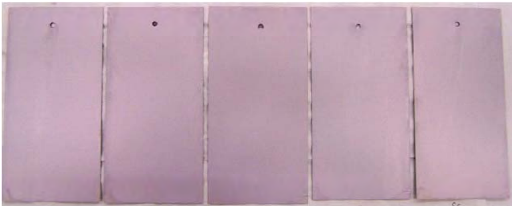
Figure 5-50 Panels S1-S5 after 2205 hours of salt fog exposure. Panel surfaces are alternating rough and smooth from S1 to S5.
