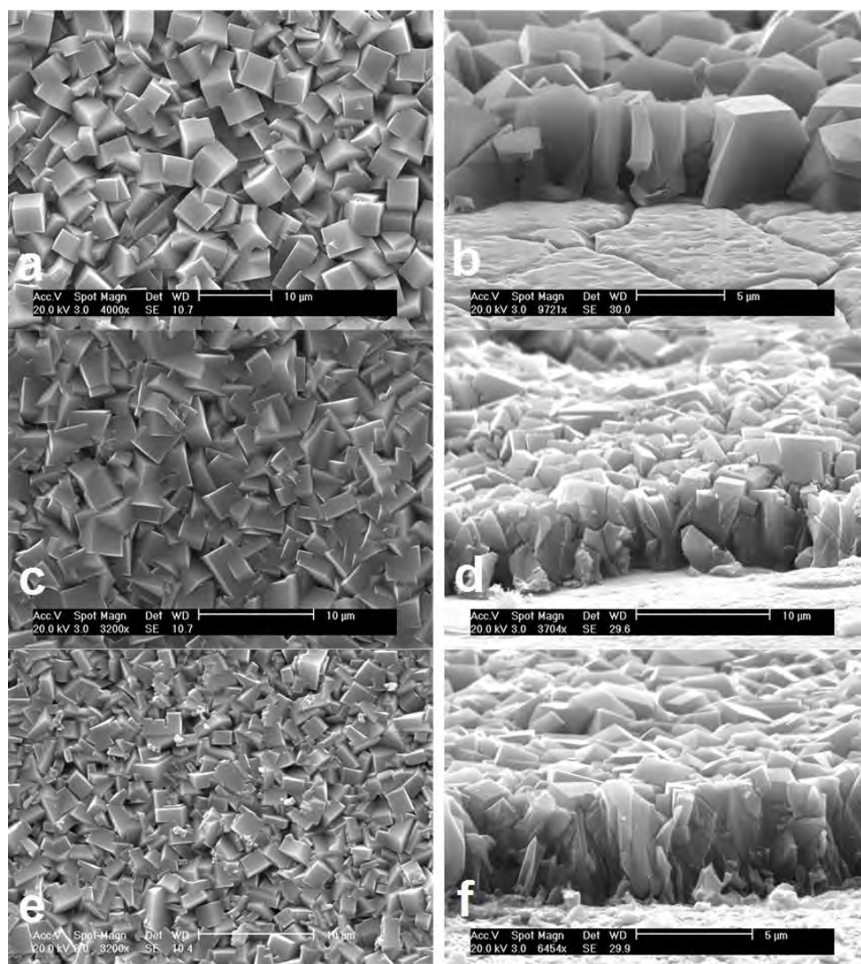
Figure 5-5 SEM images of ZSM-5 coatings (4 - 5 \mu m thick) on steels. SS304-2b (a, b); S1008 (c, d); S4130 (e, f)
