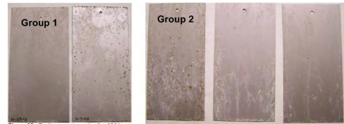
Figure 5-36 Zeolite coated panels after 336 hours of salt fog exposure
