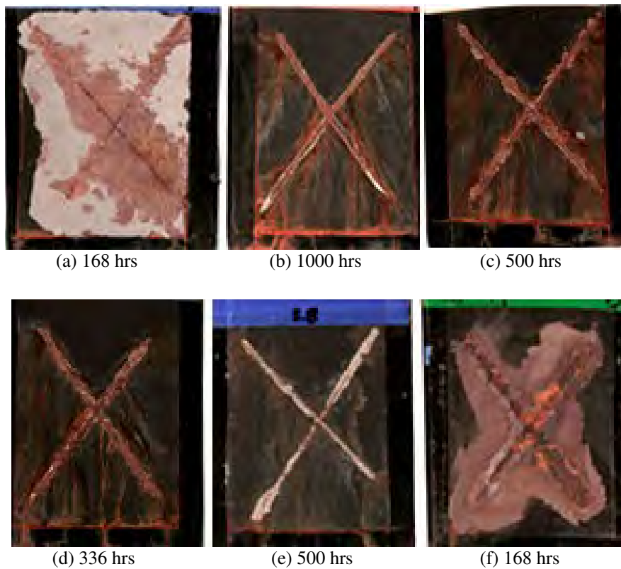
Figure 4. SST results for CRS coated with with MIL-P-23377J /MIL-C-53039A; (a) no wash primer, (b) DoD-P-15328D, (c) AU-23(A), (d) AU-23(D), (e) EPZ-0 and (f) E-11.
