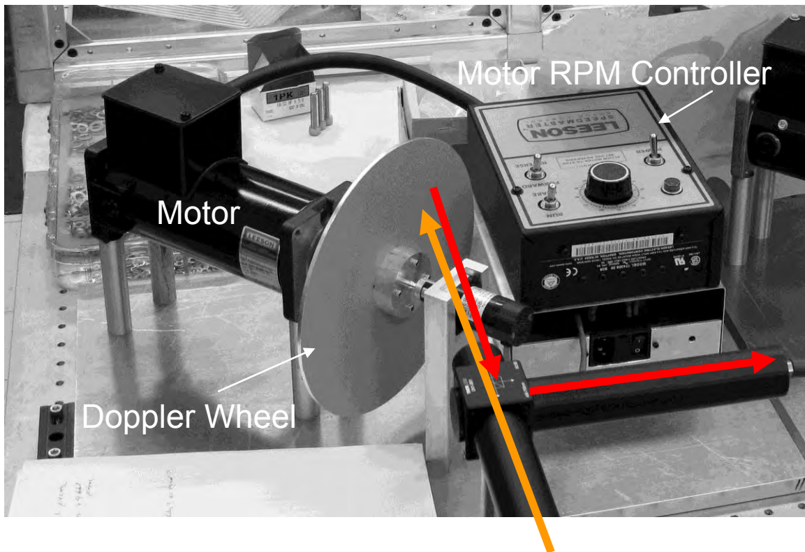
Figure 19: Doppler scene generator with simplified ray trace
