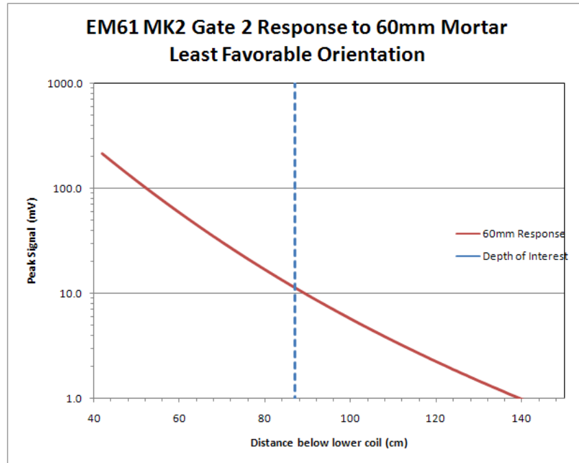
Figure 3 – EM61 MK2 gate 2 response curve for a 60mm mortar in its least favorable orientation
