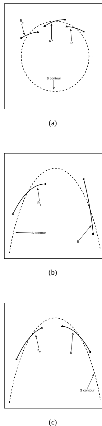
Fig. 5. (a) Sketch of a structure \mathcal{R} of R at initial time t_0 , the associated structure \mathcal{R}' of R at initial time t_0 + \tau , and the flow map image \mathcal{R}_\tau = \phi_{t_0+\tau}^{t_0}(\mathcal{R}) , illustrating the non-Lagrangian nature of the coherent structures. (b) Structure \mathcal{R} crossing an S contour with speed above the contour higher than the speed below, and flow map image \mathcal{R}_\tau after an integration time. Leading and lagging ends of \mathcal{R} and their images on \mathcal{R}_\tau are marked by a triangle and a square, respectively. (c) Same as (b) with opposite orientation of \mathcal{R} relative to the contour, leading to a rotation of \mathcal{R}_\tau .
