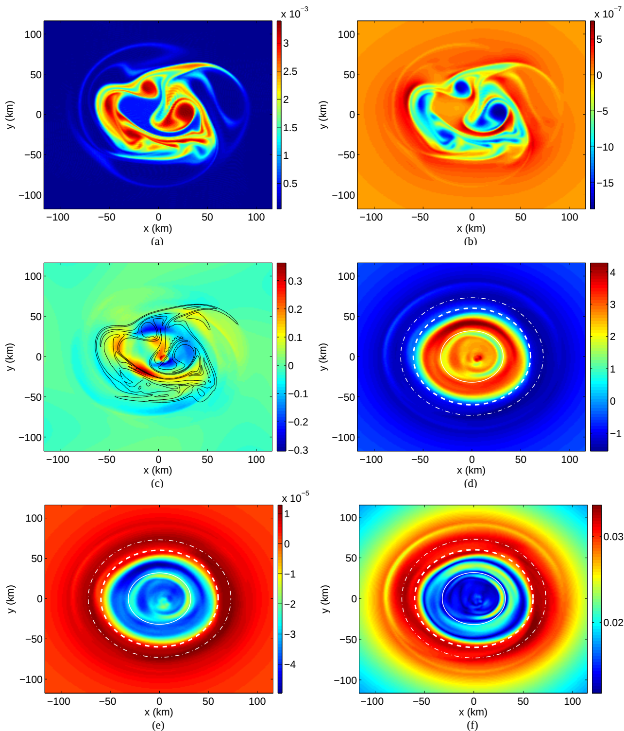
Fig. 11. (a) Relative vorticity field, (b) Q -field, (c) R -field with vorticity contours overlayed to relate structures, (d) S -field, (e) integrated Q -field \hat{Q} , and (f) FTLE-field for initial time of t_0=12 h with integration time T=1 h. The white contours in (d)–(f) mark the radius of maximum \frac{\partial \omega}{\partial r} (inner, solid), the radius of maximum tangential wind (middle, dashed), and the radius of maximum counterpropagating \frac{\partial \omega}{\partial r} (outer, dash-dot).
