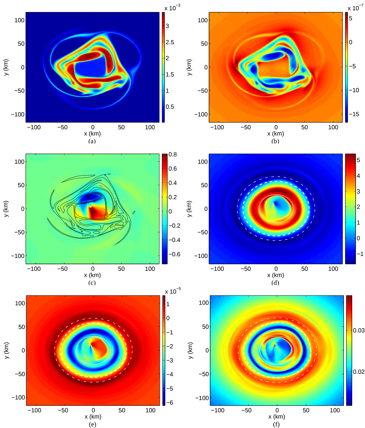
Fig. 10. (a) Relative vorticity field, (b) Q -field, (c) R -field with vorticity contours overlayed to relate structures, (d) S -field, (e) integrated Q -field \bar{Q} , and (f) FTLE-field for initial time of t_0=10 h with integration time T=1 h. The white contours in (d)–(f) mark the radius of maximum \frac{\partial \omega}{\partial r} (inner, solid), the radius of maximum tangential wind (middle, dashed), and the radius of maximum counterpropagating \frac{\partial \omega}{\partial r} (outer, dash-dot).
