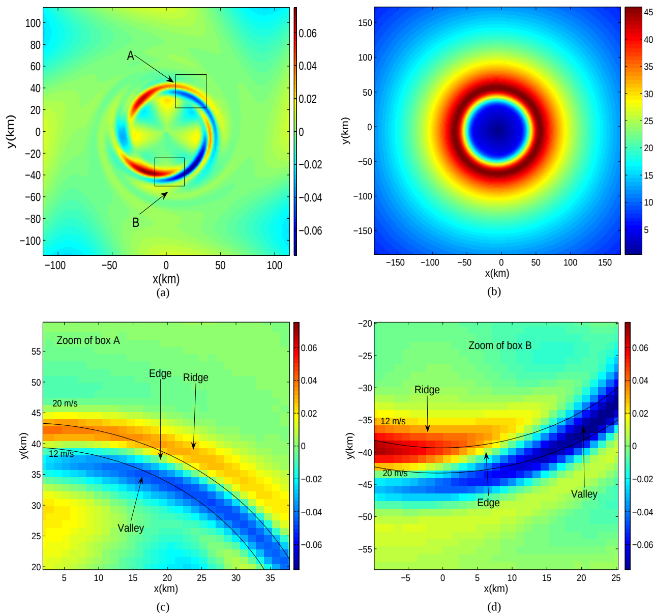
Fig. 4. (a) R -field with ridges and valleys and (b) Lagrangian speed at t_0 = 2 h. (c) Zoom of box A from R -field showing repelling edge, and (d) zoom of box B showing attracting edge. Integration time is T = 60 min. Black lines show the azimuthal velocity at the initial time.
