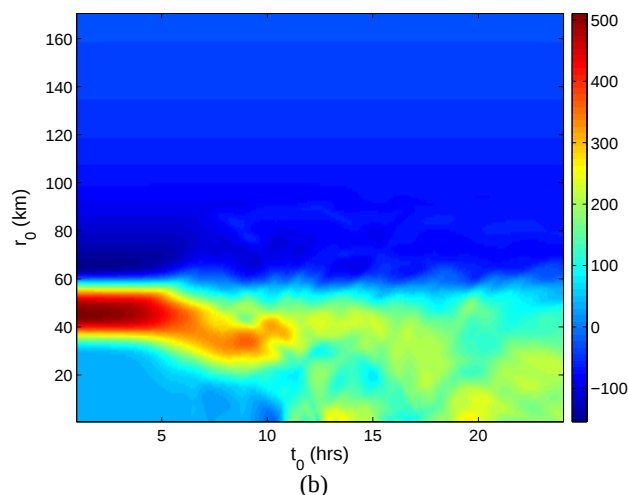
Fig. 14. Radial S -values \bar{S}(r_0, t_0) for integration times (a) 30 min and (b) 1 hr.
