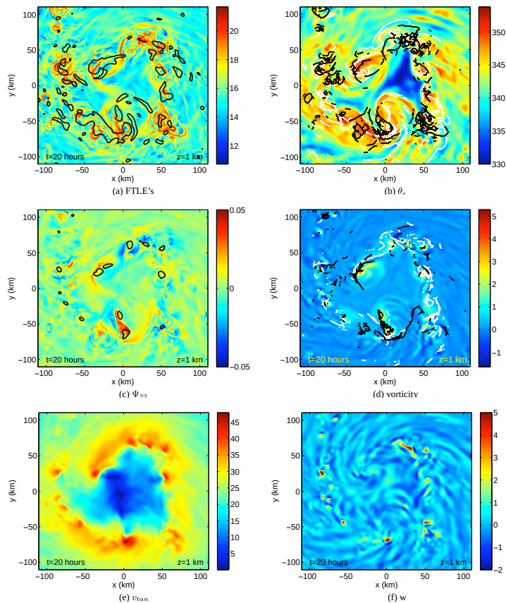
Fig. 5. Horizontal slices of Lagrangian fields and Eulerian diagnostics are compared at 20 h and 1 km height. The FTLE field (a) has ridges, which are extracted and overlaid on the \theta_e field (b) . The \Psi_{22} field (c) has ridges, which are extracted and overlaid on the \zeta field (d) . Tangential winds and vertical velocity are shown in (e) and (f) .
