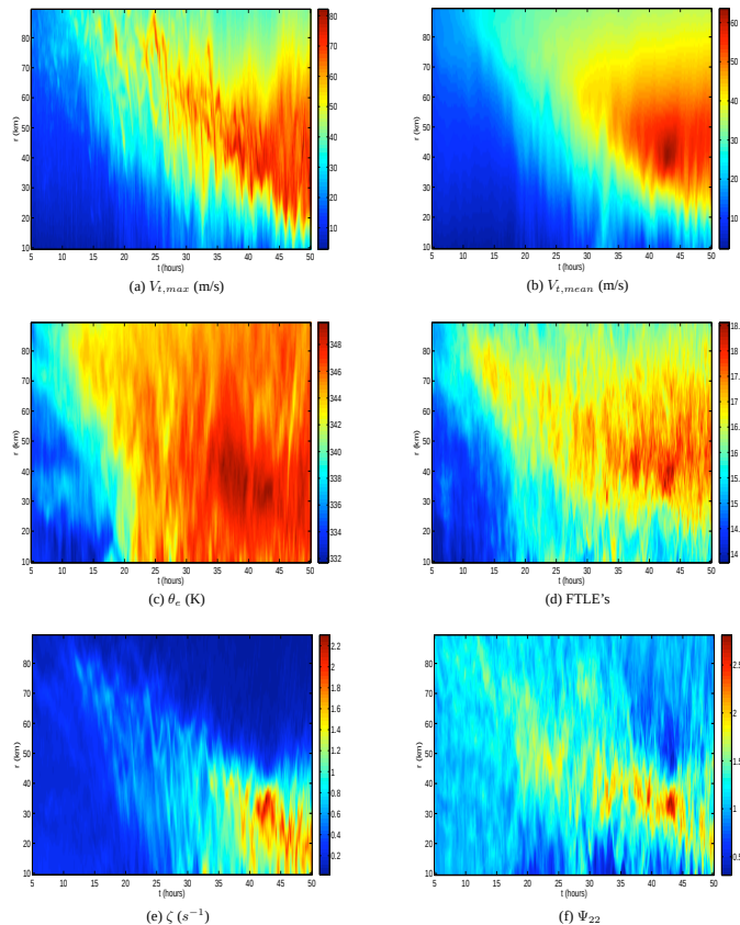
Fig. 2. Hovmöller plots (radial profile versus time) of azimuthally averaged V_{\tan, \max} (a) , V_{\tan, \text{mean}} (b) , \theta_e (c) , FTLE's (d) , \zeta (e) , and \Psi_{22} (f) . The V_{\tan, \text{mean}} , FTLE, \Psi_{22} , \theta_e , and \zeta values are averaged over the z = 40 m horizontal plane, while V_{\tan, \max} is a maximum over all heights and azimuths at each radius.
