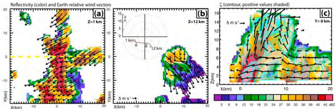
Figure 2. ELDORA analysis from 0036–0058 UTC 14 September, 2008. Horizontal plan view of radar reflectivity (color, dBZ) and wind vectors are shown at (a) 1 km and (b) 12 km altitude. (c) Reflectivity (color), relative vertical vorticity ( 4 \times 10^{-3} \text{ s}^{-1} contours, positive [cyclonic] values shaded), and wind vectors in the X-Z plane. Yellow dashed line in Figure 2a depicts the vertical cross-section in Figure 2c. Inset in Figure 2b is radar-derived velocity hodograph.
