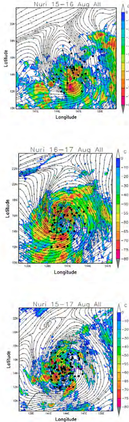
Fig. 2. Dropsonde locations for Nuri1 and Nuri2 as viewed in the co-moving frame of reference with the parent wave-like disturbance (moving approximately 7 \text{ m s}^{-1} westward). The usable drop points and co-moving streamlines at the 925 hPa level from the GFS FNL analysis are superimposed on the satellite brightness temperature. The color bar for the brightness temperature is indicated. The red and orange colors indicate the approximate cloud-top temperatures of areas of active deep convection and their associated anvil clouds. Shown are a) dropsonde locations for Nuri1 together with 925 hPa co-moving streamlines and brightness temperature at 00Z 16 August; b) dropsonde locations for Nuri2 together with 925 hPa co-moving streamlines and brightness temperature at 00Z 17 August; c) drop locations for both Nuri1 and Nuri2 translated to the 12Z 16 August brightness temperature image and co-moving streamline field, the time nearest the genesis time as declared by JTWC forecasters. The purple curve denotes the local critical latitude where the parent wave's zonal phase speed coincides with the mean zonal flow at the 925 hPa level. The dark black curve denotes the trough axis of the wave disturbance at this same level. The intersection between these two curves denotes the sweet spot of the pouch region (see Montgomery et al. (2010) for further details).
