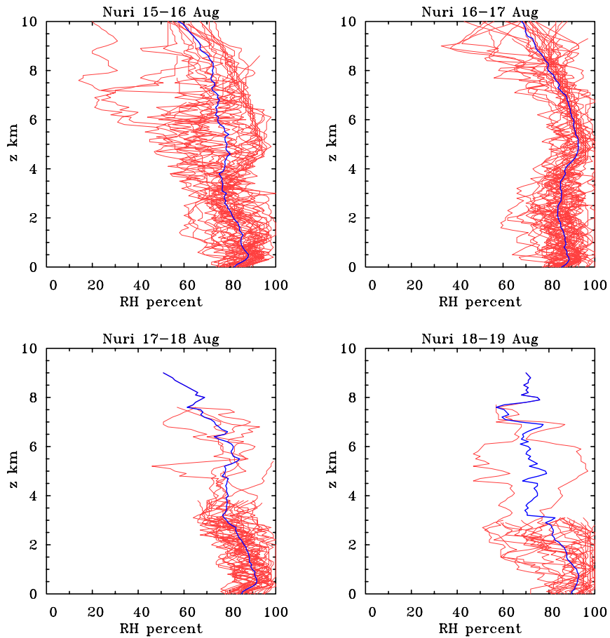
Fig. 4. Vertical profiles of relative humidity (RH) for each usable sounding on all days of Nuri. The system-average RH is depicted by the solid blue curve.
