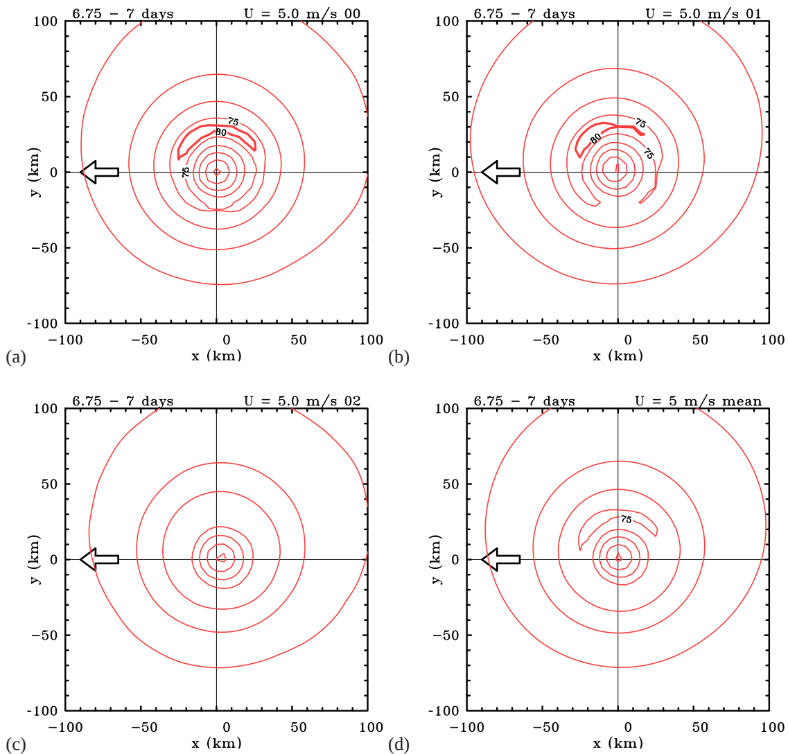
Figure 9. Contours of Earth-relative total wind speed at 850 mb averaged during the period 6\frac{3}{4} - 7 days about the centre of minimum total wind speed at this level. (a) the main experiment and (b), (c) two ensemble experiments with U = 5.0 \text{ m s}^{-1} . Panel (d) shows the average of the main and ten ensemble experiments. Contour interval 15 \text{ m s}^{-1} (thin contours). The thick contour in panels (a) and (b) has the value 80 \text{ m s}^{-1} . The arrow indicates the direction of vortex motion.
