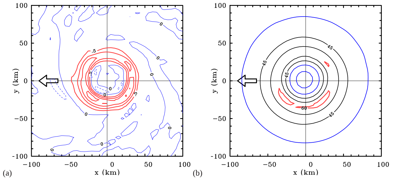
Figure 14. Contours of (a) vertical velocity, and (b) total wind speed at 850 mb averaged during the period t_4^3 - 7 days about the centre of minimum total wind speed at this level in the experiment with U = 5.0 \text{ m s}^{-1} which uses the Gayno-Seaman boundary-layer parameterization scheme. The arrow indicates the direction of vortex motion.
