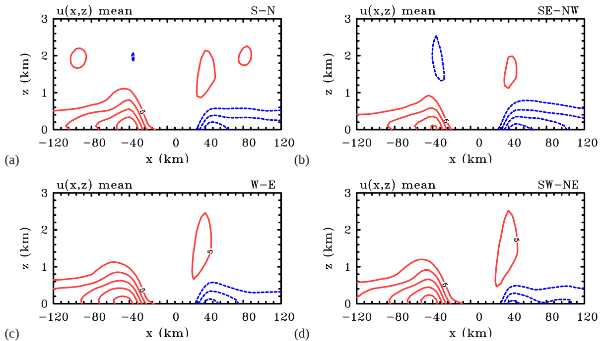
Figure 15. Height-radius cross sections showing isotachs of the wind component in different compass directions ( x ) in the co-moving frame. The data are for the control calculation with U = 5 \text{ m s}^{-1} and with the Gayno-Seaman boundary-layer scheme, and are averaged over the last 6 hours of the calculation. (a) south to north, (b) southeast to northwest, (c) west to east, (d) southwest to northeast. Contour values: 5 \text{ m s}^{-1} . Positive contours solid/red, negative contours dashed/blue.
