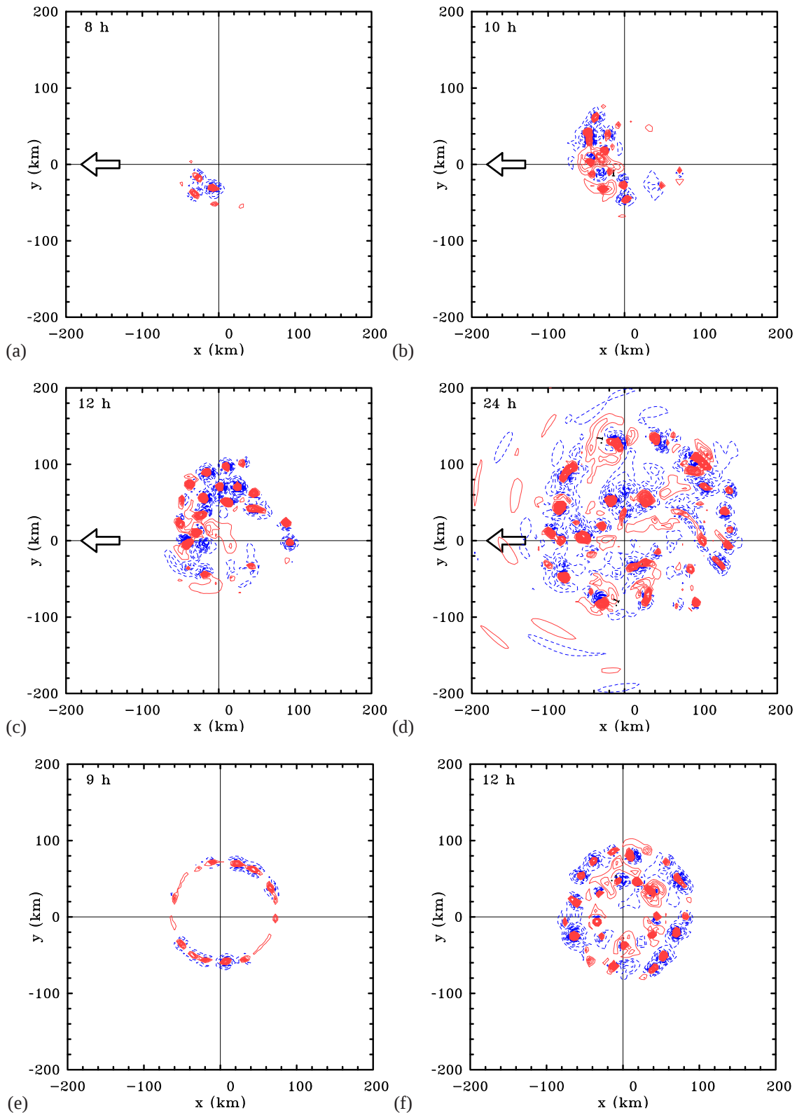
Figure 3. Contours of vertical velocity at 850 mb at times indicated in the top right of each panel during the vortex evolution. (a)–(d) for the experiment with U = 5.0 \text{ m s}^{-1} (from right to left), and (e) and (f) for the experiment with the zero background flow. Contour interval: thick contours 0.5 \text{ m s}^{-1} , thin contours 0.1 \text{ m s}^{-1} . Positive velocities (solid/red lines), negative velocities (dashed/blue lines). The arrow indicates the direction of vortex motion.
