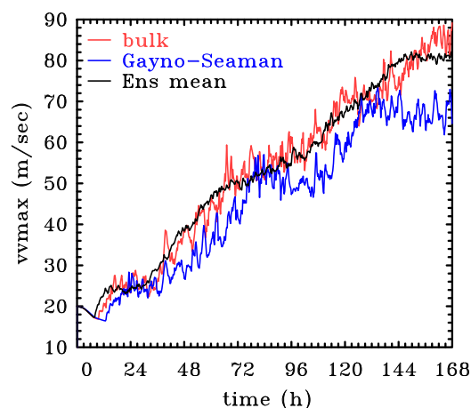
Figure 13. Time series of maximum total wind speed at 850 mb for the control experiments with U = 5.0 \text{ m s}^{-1} (bulk/red curve), the corresponding ensemble mean (Ens mean/black curve) and the experiment using the Gayno-Seaman boundary-layer scheme (blue curve).
