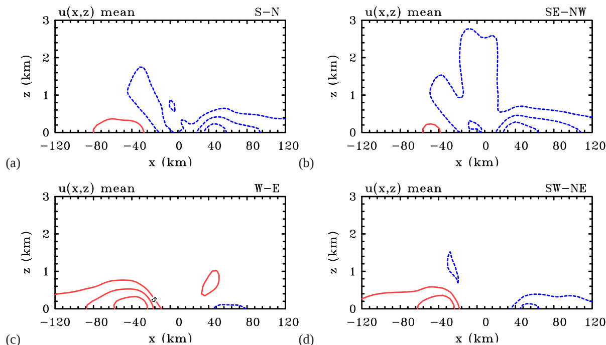
Figure 12. Height-radius cross sections showing isotachs of the wind component in different compass directions ( x ) in the co-moving frame. The data are for the control calculation with U = 5 \text{ m s}^{-1} and a sea surface temperature of 25^\circ\text{C} , and are averaged over the last 6 hours of the calculation. (a) south to north, (b) southeast to northwest, (c) west to east, (d) southwest to northeast. Contour values: 5 \text{ m s}^{-1} . Positive contours solid/red, negative contours dashed/blue.
