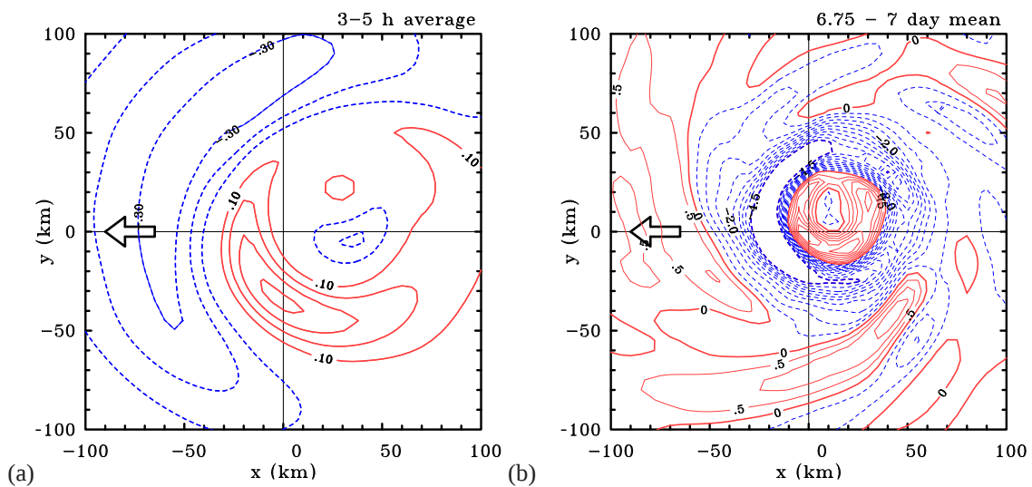
Figure 6. Contours of divergence at 500 m at for the experiment with U = 5.0 \text{ m s}^{-1} and a sea surface temperature of 25^\circ\text{C} : (a) between 3-5 hours (contour interval 1 \times 10^{-5} \text{ s}^{-1} ). (b) between 6\frac{3}{4} - 7 days (contour interval: thick contours 5 \times 10^{-4} \text{ s}^{-1} , thin contours 5 \times 10^{-5} \text{ s}^{-1} . Positive contours (solid/red) and negative values (dashed/blue). The arrow indicates the direction of vortex motion.
