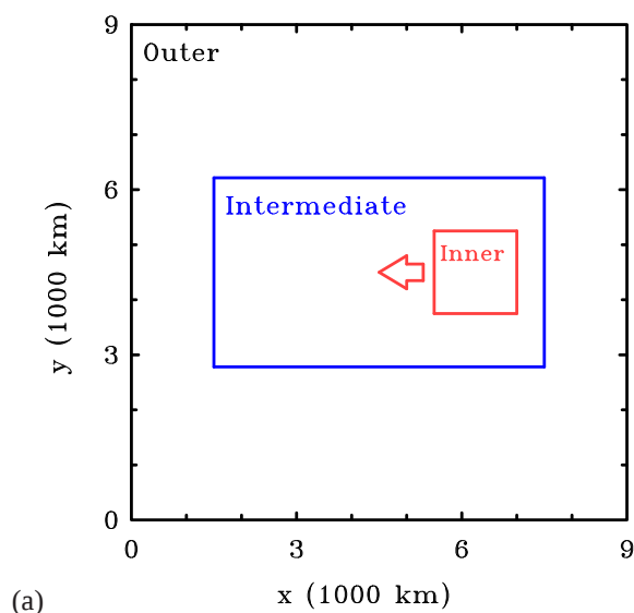
Figure 1. Configuration of the three model domains. The inner domain is moved from east to west (the negative x -direction) at selected times to keep the vortex core away from the domain boundary.
