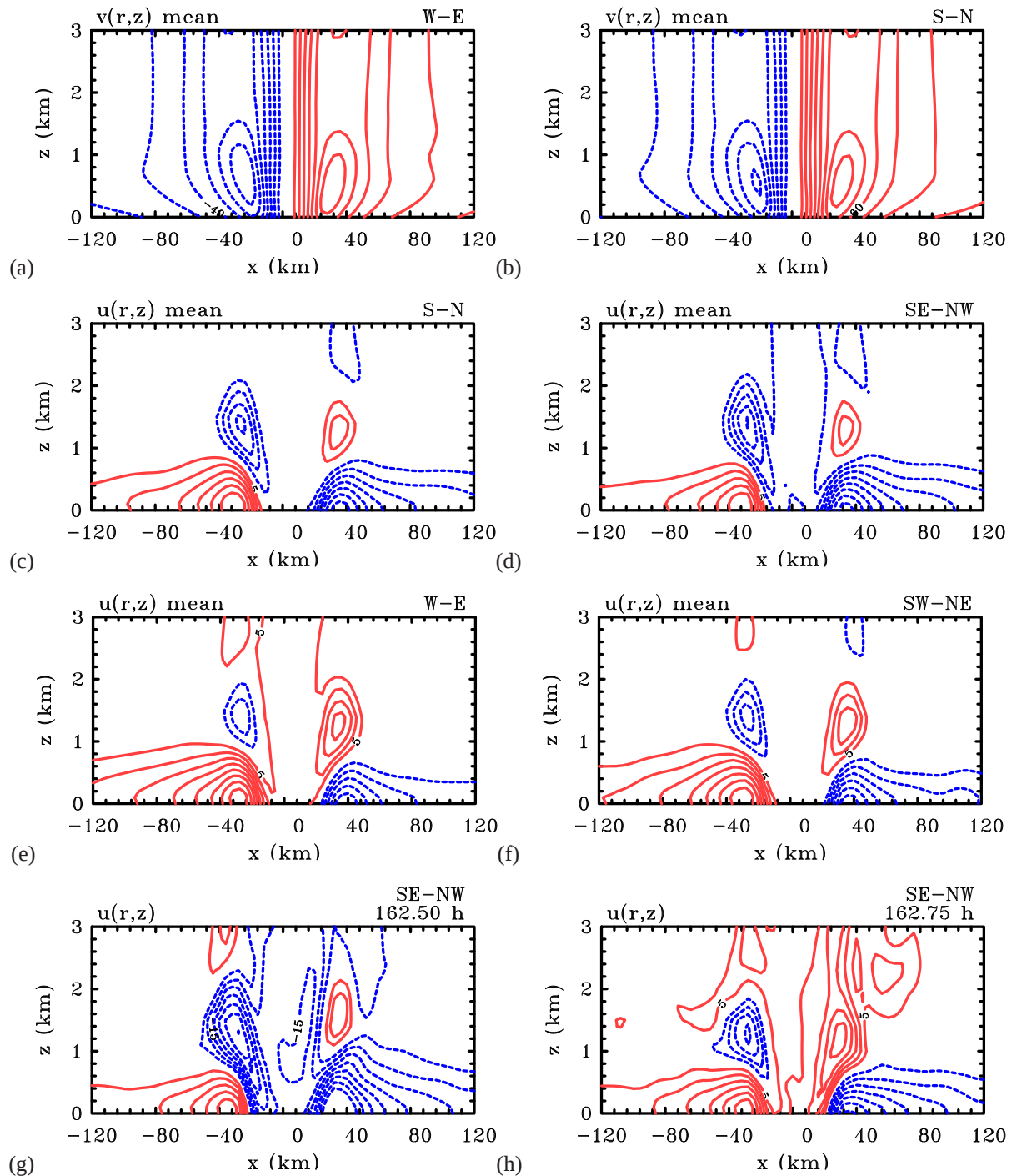
Figure 11. Height-radius cross sections showing the isotachs of the wind components in and normal to different compass directions ( x ) in the co-moving frame. The data are for the control calculation with U = 5 \text{ m s}^{-1} and are averaged over the last 6 hours of the calculation. Normal component to the cross section: (a) west to east, (b) south to north. Component in the cross section: (c) south to north, (d) southeast to northwest, (e) west to east, (f) southwest to northeast. Panels (g) and (h) show the radial wind at two particular times, 15 minutes apart, during the last six hours. Contour values: 10 \text{ m s}^{-1} for normal (tangential) wind, 5 \text{ m s}^{-1} for the wind component in the cross section. Positive contours are denoted by solid/red and negative contours are denoted by dashed/blue.
