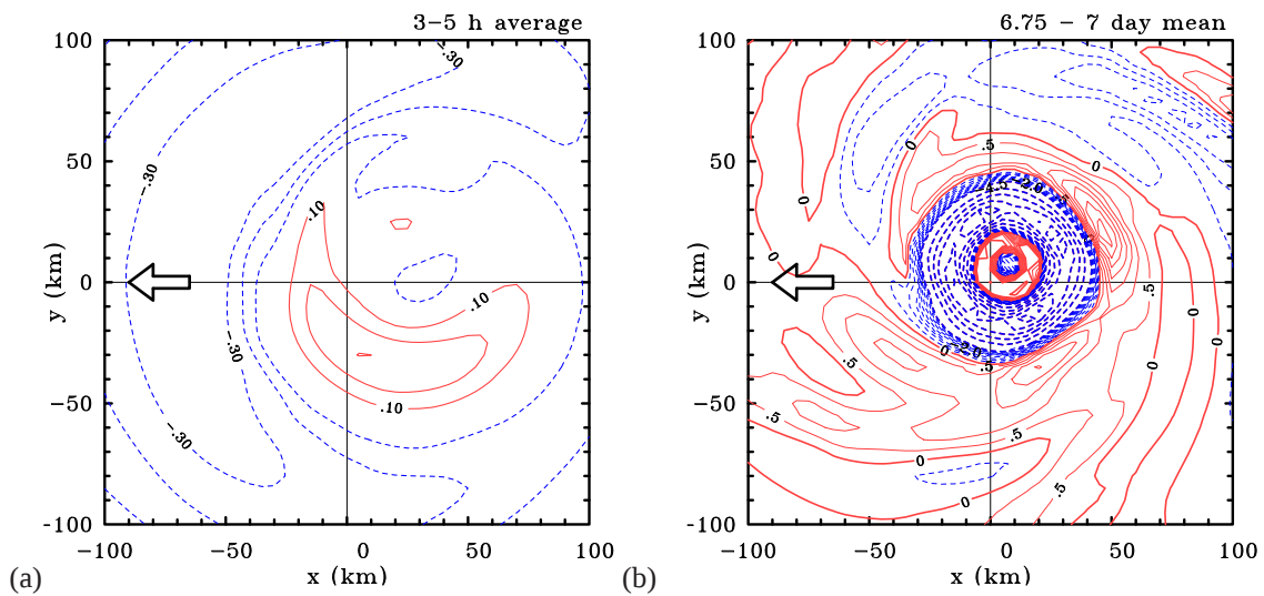
Figure 5. Contours of divergence at 500 m at for the experiment with U = 5.0 \text{ m s}^{-1} : (a) between 3-5 hours (contour interval 1 \times 10^{-5} \text{ s}^{-1} . Positive contours (solid/red) and negative values (dashed/blue).) and (b) between 6\frac{3}{4} - 7 days (contour interval: thick contours 5 \times 10^{-4} \text{ s}^{-1} , thin contours 5 \times 10^{-5} \text{ s}^{-1} . Positive contours (solid/red) and negative values (dashed/blue)). The arrow indicates the direction of vortex motion.
