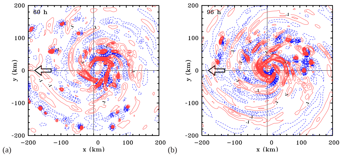
Figure 4. Contours of vertical velocity at 850 mb at (a) 60 hours, and (b) 96 hours, during the vortex evolution for the experiment with U = 5.0 \text{ m s}^{-1} (from right to left). Contour interval: thick contours 0.5 \text{ m s}^{-1} , thin contours 0.1 \text{ m s}^{-1} . Positive velocities (solid/red lines), negative velocities (dashed/blue lines). The arrow indicates the direction of vortex motion.
