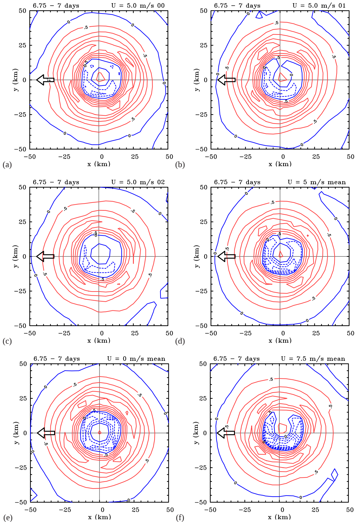
Figure 8. Contours of vertical velocity at 850 mb averaged during the period 6.75 – 7 days about the centre of minimum total wind speed at this level in the experiments with U = 5.0 \text{ m s}^{-1} . (a) The main experiment; (b) and (c) two ensemble experiments, and (d) the average of the main and ten ensemble experiments. For comparison, panels (e) and (f) show the mean fields (main experiment plus four ensembles) for the experiment with no background flow and that for U = 7.5 \text{ m s}^{-1} , respectively. Contour interval 0.5 \text{ m s}^{-1} . Positive velocities (solid/red lines), negative velocities (dashed/blue lines). The arrow indicates the direction of vortex motion.
