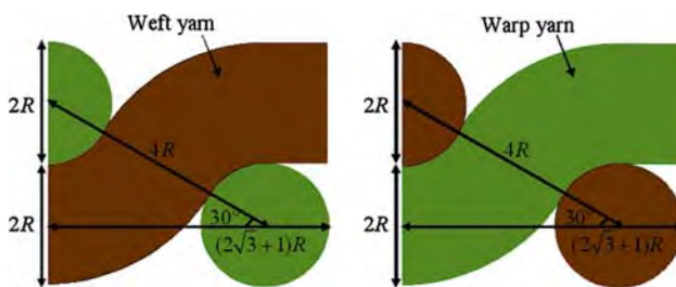
Fig. 1 Cross-sectional views of a twill woven fabric
