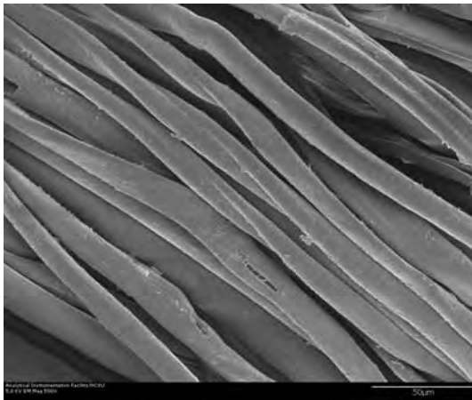
Fig. 2 SEM micrograph of a NyCo multifilament yarn ( \times 500 )
