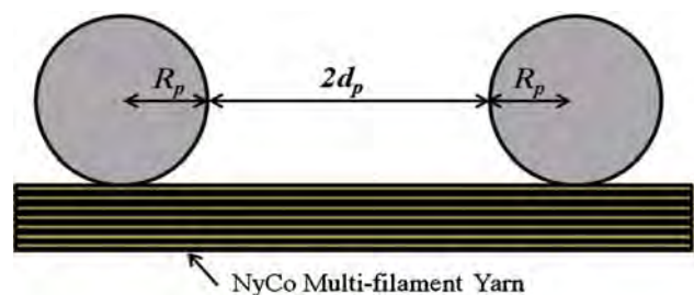
Fig. 4 Two adjacent protuberances on a NyCo surface
