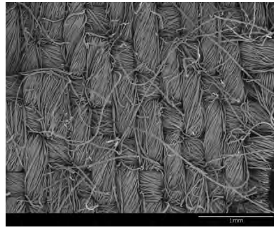
Fig. 3 SEM micrograph of a multifilament twill woven fabric ( \times 25 )
