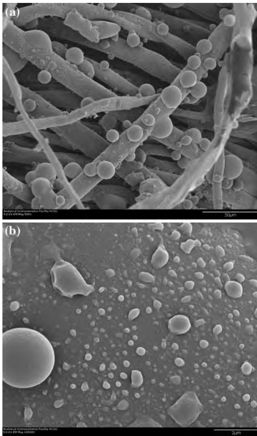
Fig. 5 SEM micrographs of fluorosilane-treated on NyCo a \times 500 and b \times 10,000
