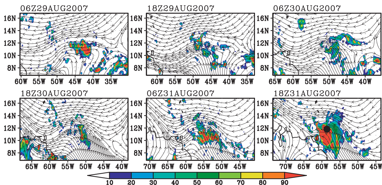
FIG. 1. Streamlines of the 2.5-day low-pass filtered 850-hPa flow from ECMWF analyses in the earth-relative frame of reference from 0600 UTC 29 Aug to 1800 UTC 31 Aug. Shading indicates TRMM 3-h accumulated precipitation ( \text{mm day}^{-1} ). The genesis location is indicated by the black dot in the final panel.
