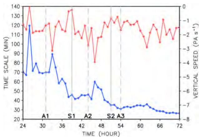
Figure 16. The evolution of the azimuthal-mean vertical velocity \bar{w} [ \text{Pa s}^{-1} ] (dashed line, red in the online article) and azimuthal-mean filamentation time-scale \tau_{\text{fil}} [min] (solid line, blue in the online article) at the 80 km radius at 850 hPa. This figure is available in colour online at wileyonlinelibrary.com/journal/qj
