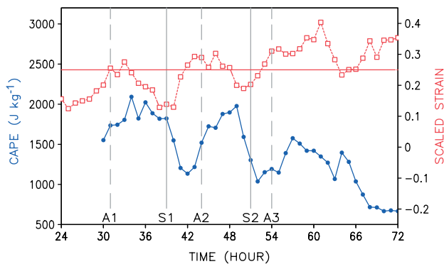
Figure 17. Evolution of azimuthal-mean CAPE (solid line with filled circles) [ \text{J kg}^{-1} ] and rate of strain scaled by relative vorticity \gamma = S/\zeta (dashed line with squares) at a radius of 50 km. This figure is available in colour online at wileyonlinelibrary.com/journal/qj
