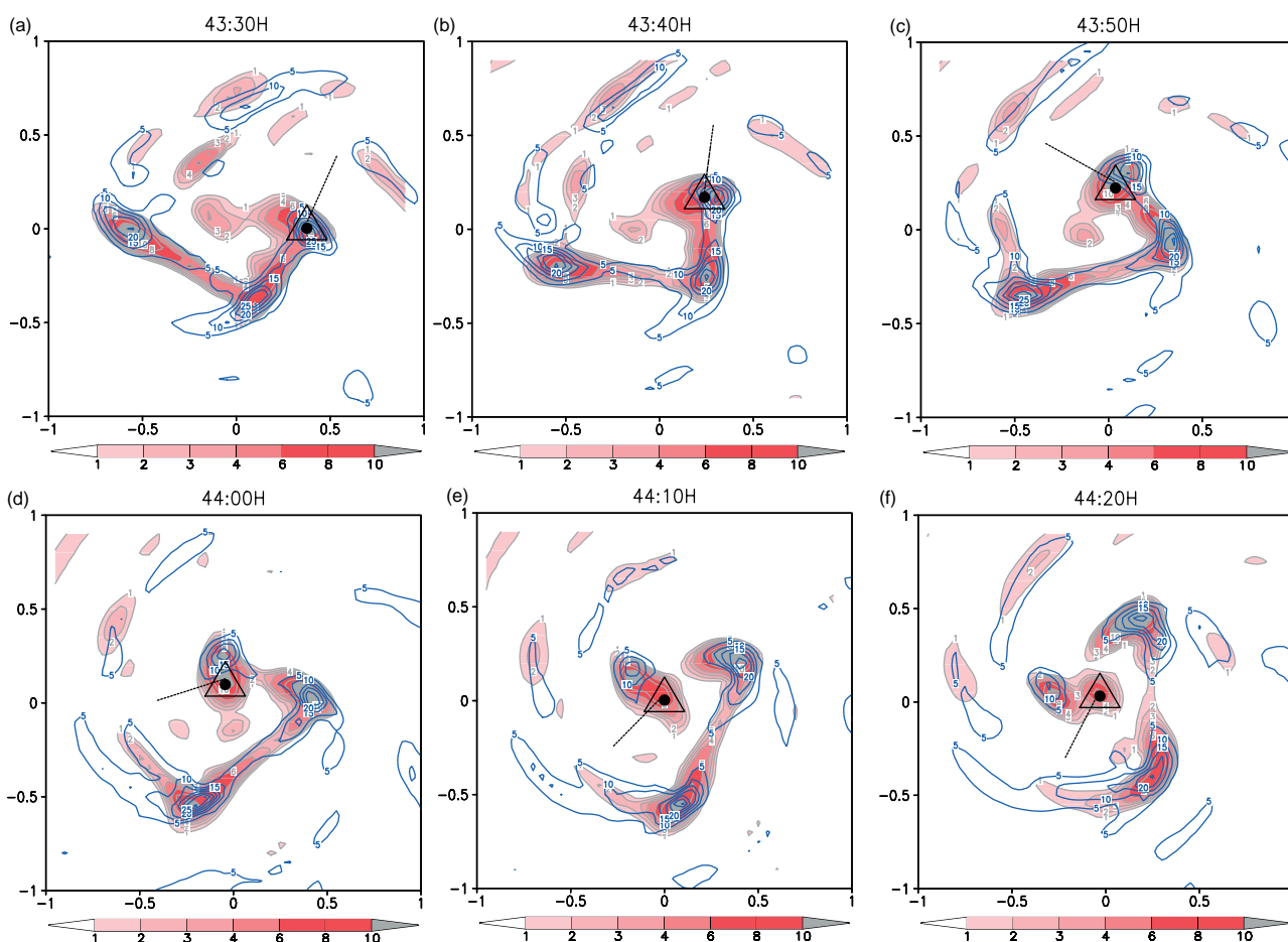
Figure 11. Local PV maxima at 850 hPa represented by -\nabla^2(\text{PV}) [ 10^{-8} \times \text{PVU m}^{-2} ] (shaded regions represent positive anomalies). Labels on the horizontal and vertical axes show distance in degrees from the vortex centre in the zonal and meridional directions, respectively. Contours are vertical velocity in pressure coordinates [ -1 \text{ Pa s}^{-1} ]. Dotted lines ending with filled circles inside triangles mark the positions of a tracked local PV maximum. The figures show the fields at 10 min intervals after 43:30 h of integration, during the transition from the symmetric to the asymmetric phase. (a) 43:30 h, (b) 43:40 h, (c) 43:50 h, (d) 44:00 h, (e) 44:10 h, (f) 44:20 h. This figure is available in colour online at wileyonlinelibrary.com/journal/qj
