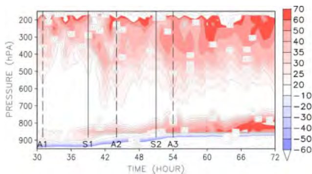
Figure 12. Evolution of the vertical gradient of the mean tangential wind \partial\bar{v}/\partial p [ 10^{-3} \times \text{m s}^{-1} \text{Pa}^{-1} ] averaged across the eyewall region (from 10–50 km). This figure is available in colour online at wileyonlinelibrary.com/journal/qj
