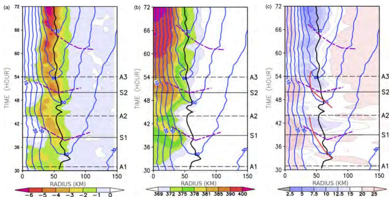
Figure 7. Radius–time plots for (a) radial gradient of mean PV \overline{\partial \overline{PV}}/\partial r [ 10^{-4} \times \text{PVU m}^{-1} ] at 850 hPa, with negative values shaded; (b) \theta_e [K] at 850 hPa; (c) CAPE [ 10^{-2} \times \text{J kg}^{-1} ]. Solid contours (blue in the online article) and dashed tilted lines (purple in the online article) show the same features as in Figure 6. Bold solid black lines show the RMW at 850 hPa. Two curved solid lines (red in the online article) in (c) mark the axes of maximum \overline{\omega} . This figure is available in colour online at wileyonlinelibrary.com/journal/qj
