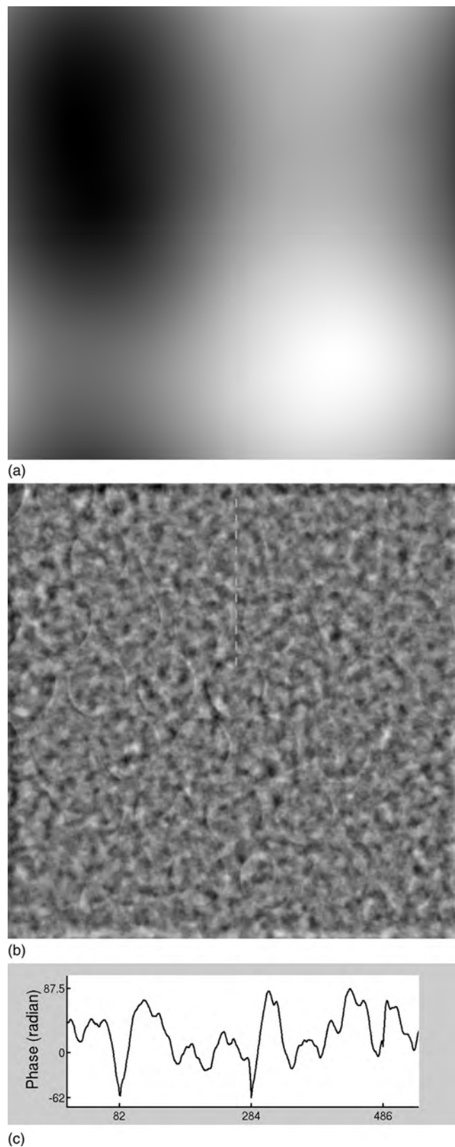
FIG. 4. Retrieved phase maps of the bubble wrap. (a) With the TIE-based method. (b) With the TIE-based method and Tikhonov regularization. (c) Profile of the retrieved phase values along the marked line on (b).
