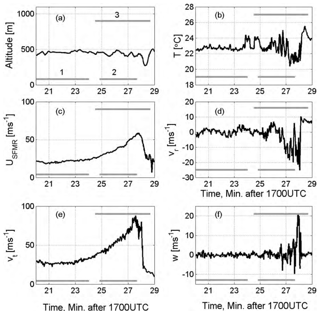
FIG. 1. Plots of (a) aircraft altitude, (b) temperature, (c) surface wind speed, (d) radial wind velocity, (e) tangential wind velocity, and (f) vertical velocity during Hurricane Hugo at 1720–1729 UTC 15 Sep 1989. The gray lines denote the three time intervals investigated.
