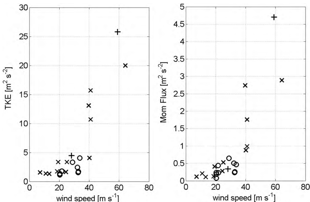
FIG. 9. Plots of TKE and momentum flux as a function of the mean wind speed at the flight level in Hurricanes Allen ( \times ), Hugo ( + ), and Frances ( \circ ).
