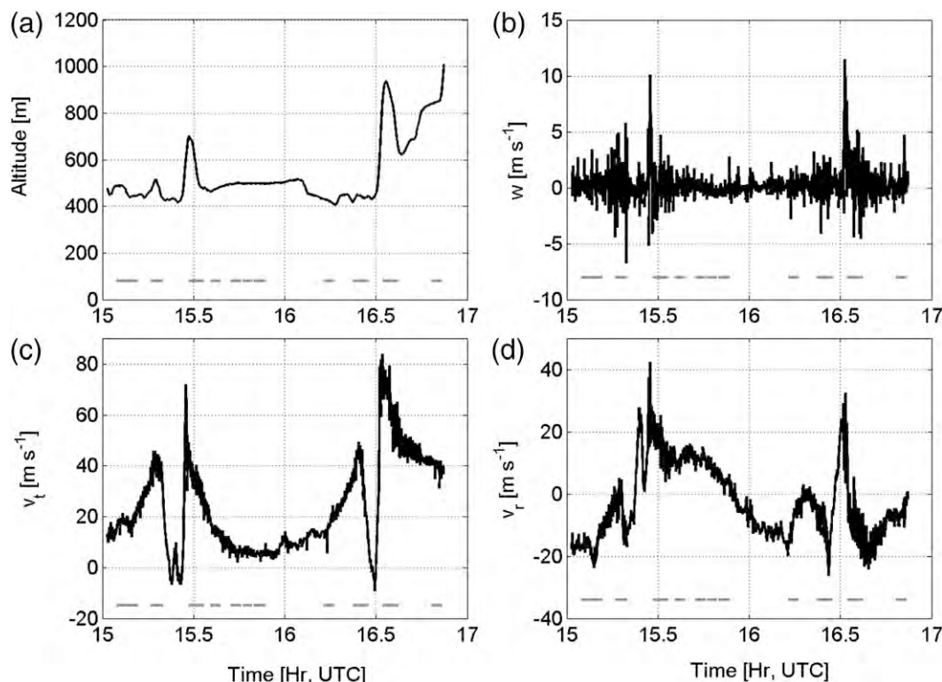
FIG. 3. Plots of (a) aircraft altitude, (b) vertical velocity, (c) tangential wind velocity, and (d) radial wind velocity during Hurricane Allen at 1501–1650 UTC 6 Aug 1980. The gray lines denote the time intervals investigated.
