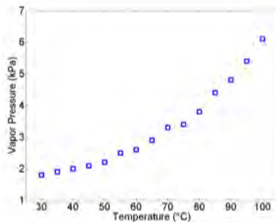
Figure 13. Dependence of vapor pressure on temperature for a fuel used in EC-1
