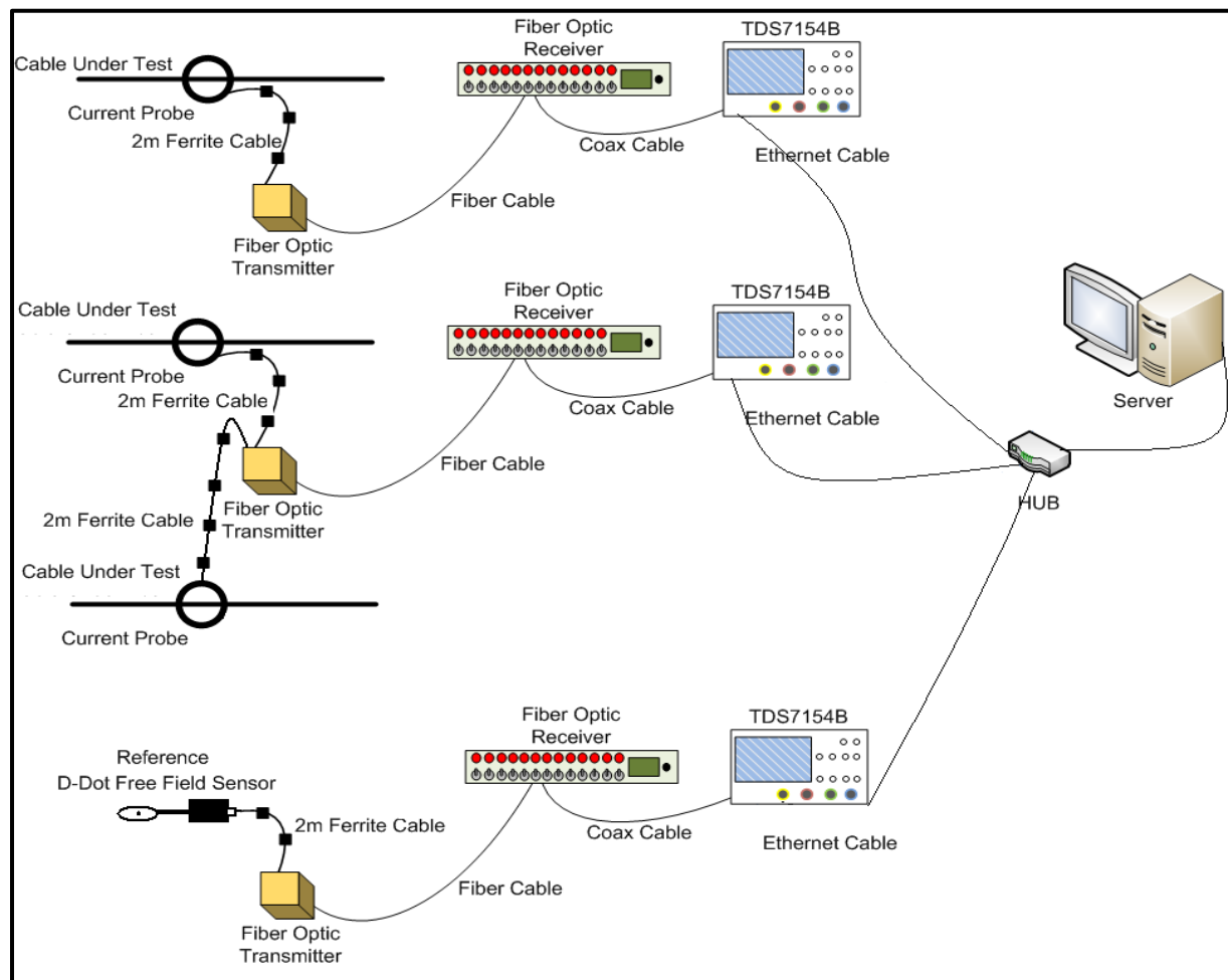
Figure 2. Data acquisition system.
