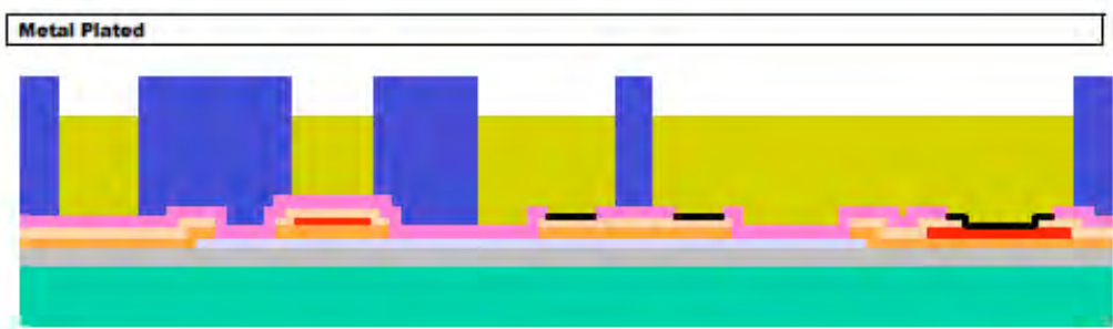
FIGURE 1.11. Nickel is electroplated to a nominal thickness of 20µm into the patterned resist stencil. A 0.5µm gold layer is then immediately electroplated on top of the nickel layer. This forms the Metal layer.
