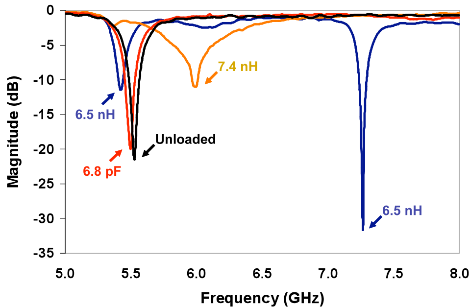
Figure 22: Measured return loss of loaded and unloaded 5.5 GHz patch antennas
