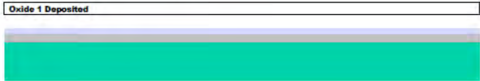
FIGURE 1.2 A 2µm thick oxide (Isolation Oxide) is grown on the surface of the starting n-type (100) silicon wafer. This is followed by deposition of a 0.5µm thick sacrificial phosphosilicate glass (PSG) layer (Oxide 1).
