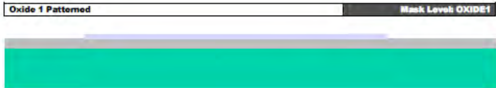
FIGURE 1.3 The wafers are coated with UV-sensitive photoresist and lithographically patterned by exposing to UV light through the first level mask (OXIDE1), and then developing it. The photoresist in exposed areas is removed, leaving behind a patterned photoresist mask for etching. Wet chemical etching is used to remove the unwanted sacrificial PSG. After the etch, the photoresist is chemically stripped. This method of patterning the wafers with photoresist, etching and stripping the remaining photoresist is used repeatedly in the MetalMUMPs process.
