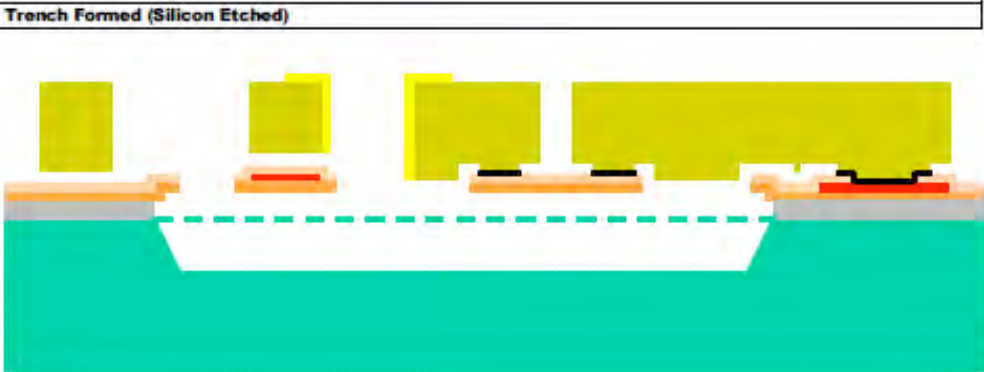
FIGURE 1.17. In the final step of the release process, a KOH silicon etch is used to form a 25µm deep trench in the silicon substrate in the areas defined by the OXIDE1 and NITR1HOLE mask levels.
