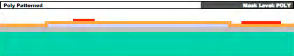
FIGURE 1.5. The wafers are coated with photoresist and the second level (POLY) is lithographically patterned. Reactive ion etching (RIE) is used to remove the unwanted polysilicon. After the etch is completed, the photoresist is removed.
