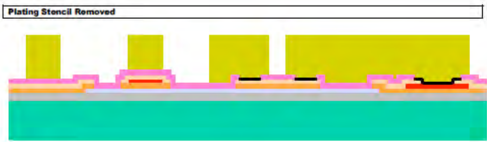
FIGURE 1.12. The photoresist stencil is then chemically removed.
