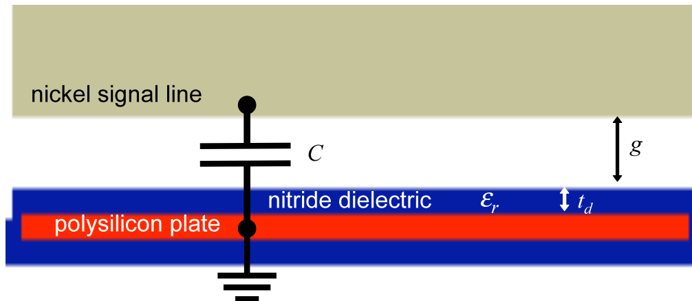
Figure 31: Diagram of MEMS capacitor, close up side view
