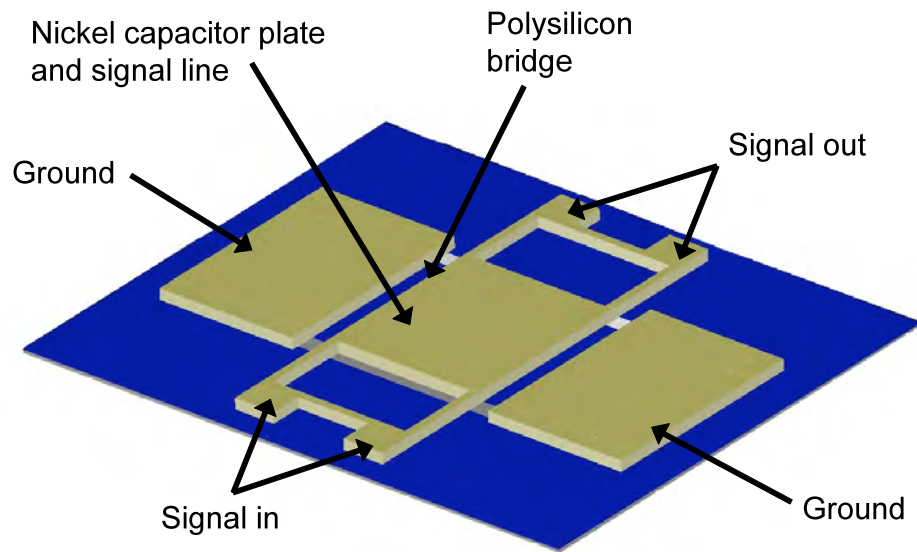
Figure 29: Diagram of MEMS capacitor, isometric view
