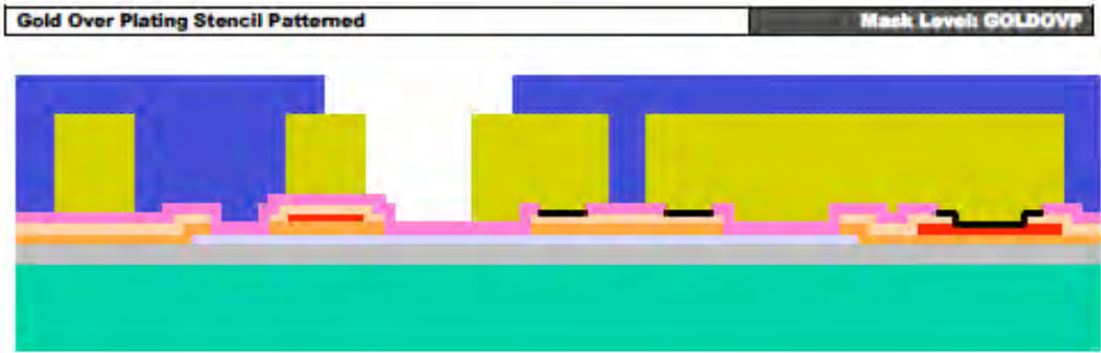
FIGURE 1.13. The wafers are coated with photoresist and patterned with a “bloated” version of the sixth mask level (GOLDOVP) to remove Plating Base in the regions where Sidewall Metal is desired. The Plating Base is chemically removed from the unpatterned regions, and the photoresist is stripped. The wafers are coated with photoresist and patterned with an “un-bloated” version of the sixth mask level (GOLDOVP) to define a resist stencil in the regions of Metal where electroplated Sidewall Metal is desired.
