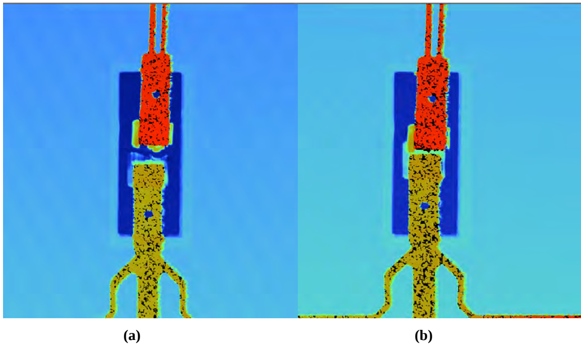
Figure 44: (a) Wyko rendering of bridge structure at 0 V and (b) at a 50 V bias voltage
