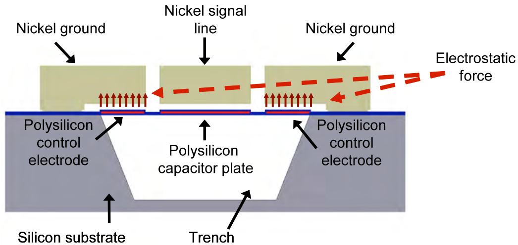
Figure 30: Diagram of MEMS capacitor, side view
