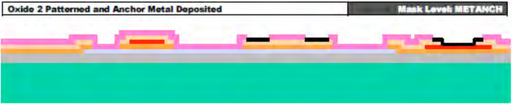
FIGURE 1.9. The wafer is coated with photoresist and the fourth mask level (METANCH) is lithographically patterned. The Oxide 2 is wet etched and a thin metal layer (Anchor Metal) consisting of 10nm Cr + 25nm Pt is deposited. A liftoff process is used to remove the photoresist and leave Anchor Metal only in the bottom of the Oxide 2 openings formed from the METANCH mask level.
