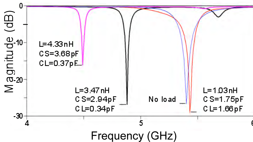
Figure 58: Simulated return loss rectangular patch antenna loaded with variable \Pi network
