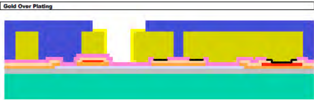
FIGURE 1.14. A 1-3µm gold layer (Sidewall Metal) is electroplated using the GOLDOVP photoresist mask as a stencil.
