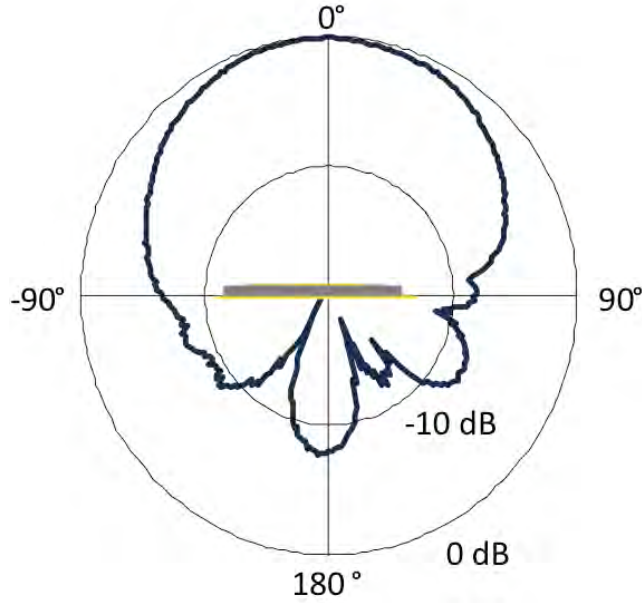
Figure 4: Radiation pattern of fabricated 5.53 GHz patch antenna
