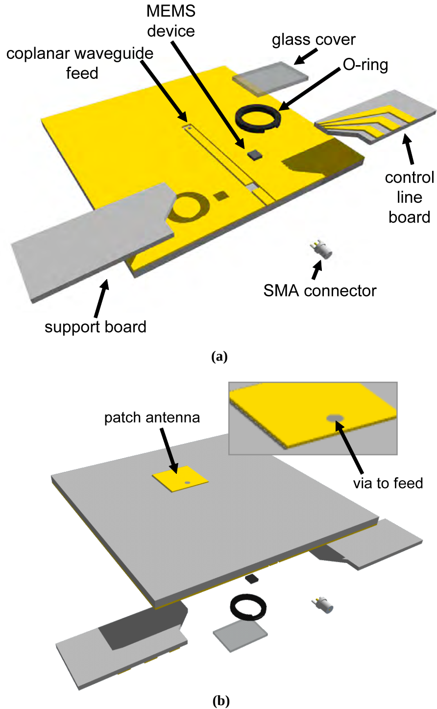
Figure 48: Diagram of (a) back and (b) front of MEMS-tuned antenna
