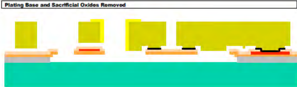
FIGURE 1.16. Plating Base is chemically stripped in the first step of the release process. In the second step of the release process, a 49% HF solution is used to remove the PSG sacrificial layers (Oxide 1 and Oxide 2) and the Isolation Oxide layer over the trench areas.
