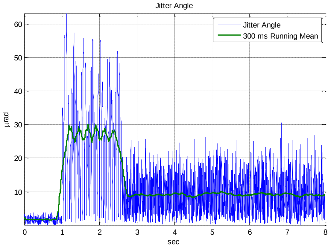
Figure 29. Jitter Angle for PSM PI Control for 10 Hz Vibration
