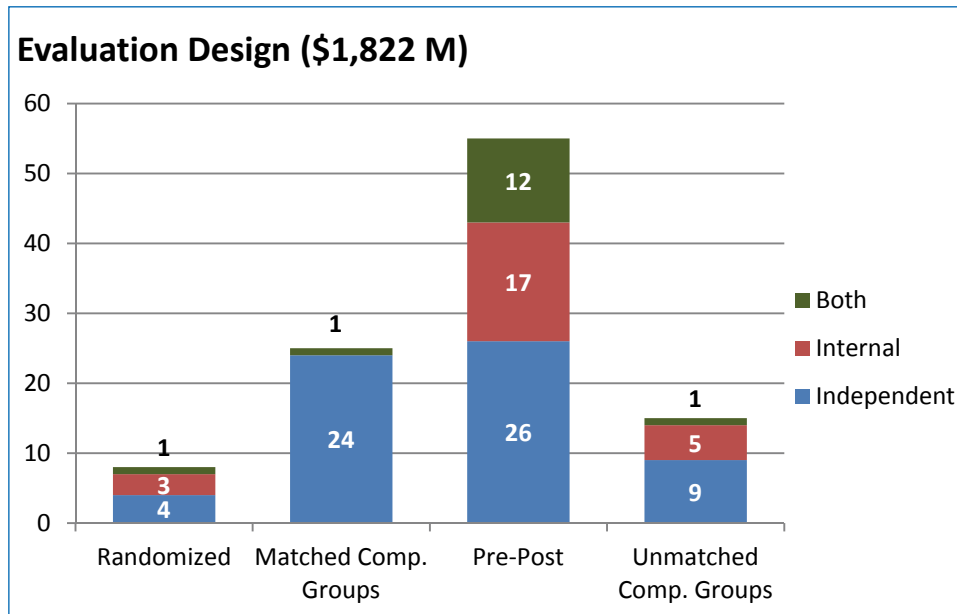
Figure 18: Evaluation Design
