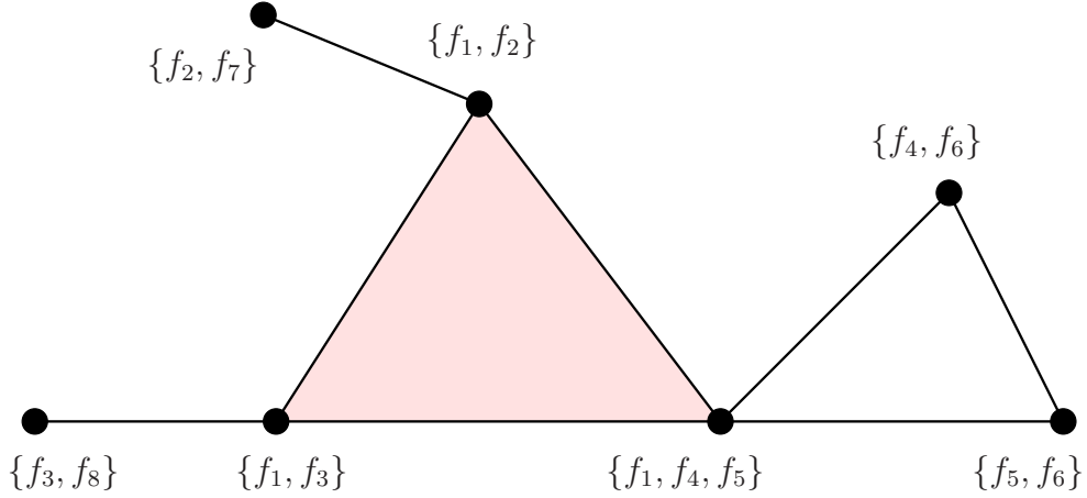
Fig. 2. An illustration of an MR-MC network and the constructed simplicial complex. The parameters within the braces are the channels which each node can access. In the communication graph derived from the network, a link exists between two nodes if and only if two nodes are within each other's transmission range and they share at least one common channel. Notice that a clique in the communication graph may not be a clique in the MR-MC network (correspondingly, a simplex in the simplicial complex), e.g., the three nodes of the right empty triangle (they do not share a common channel).
