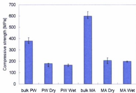
Fig.10 Compressive strength after impact of plain woven and multi-axial knitted CFRP under dry and wet condition.
