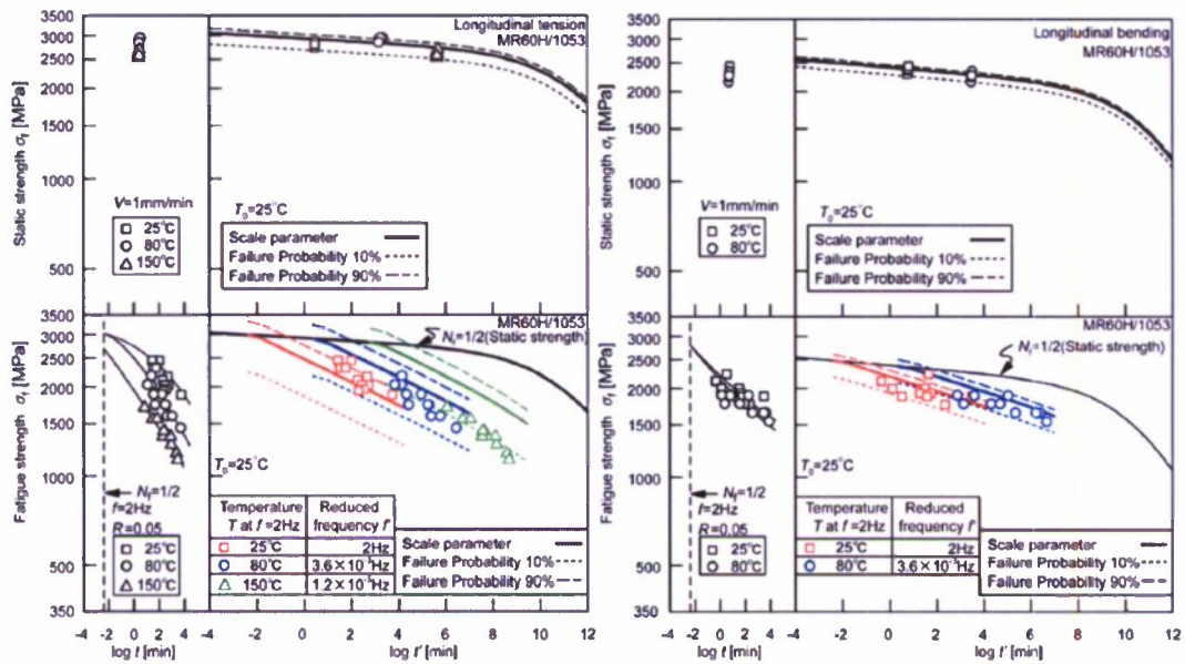
Figure 7 Master curves of tensile and bending static and fatigue strengths in the longitudinal direction of unidirectional CFRP
