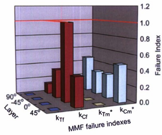
Figure 11 Judgment of initial failure of OHC for QIL under static loading ( T=25^{\circ}\text{C} , t'=1\text{ min} )
