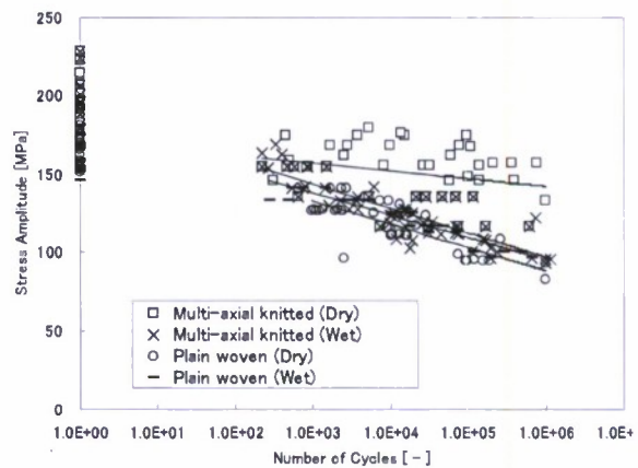
Fig.11 Fatigue strength under water absorption condition of plain woven and multi-axial knitted CFRP laminates
