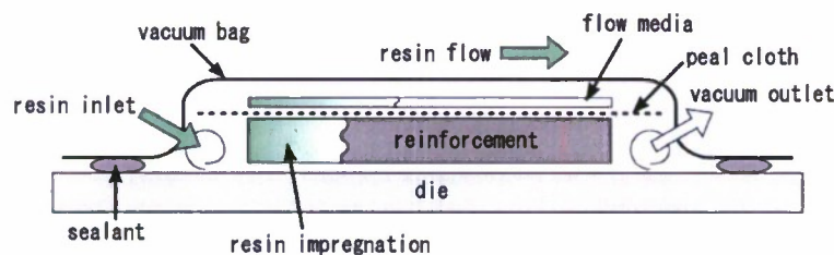
Fig.3 Schematic of vacuum assisted resin transfer molding (VARTM) setup
