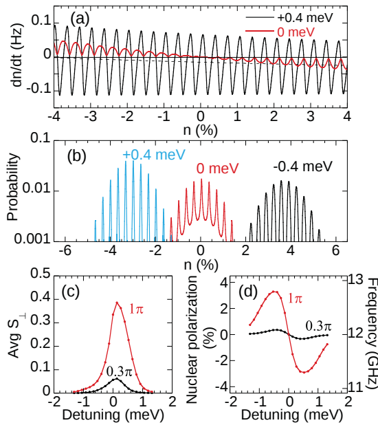
FIG. 7. (Color online) (a) Calculated dn/dt versus n for \pi pulses at zero and +0.4 meV detuning. The dashed line is the detuned data smoothed over the oscillations. (b) Calculated P(n) versus n for \pi pulses at zero and \pm 0.4 meV detuning. [(c) and (d)] Calculated average precessing spin (c) amplitude and (d) frequency as a function of pulse detuning for 0.3\pi and \pi pulses.
