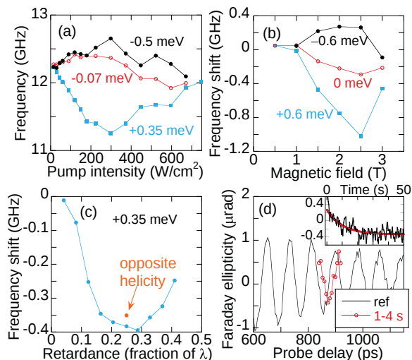
FIG. 4. (Color online) [(a)–(c)] Change in e -spin precession frequency as a function of (a) pump intensity at 2 T, circular pump polarization; (b) magnetic field at 600 W/cm 2 , circular polarization; and (c) pump polarization at 3 T, 220 W/cm 2 . A retardance of \lambda/4 corresponds to circular and 0 or \lambda/2 correspond to linear. (d) TRFE taken 1–4 s after suddenly reducing the pump intensity from 300 to 30 W/cm 2 . For the “ref” data the pump intensity had been at 30 W/cm 2 for many minutes. The inset shows the slow change in signal at 850 ps delay due to decay of the nuclear polarization.
