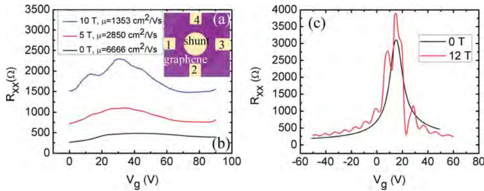
FIG. 1. (Color online) (a) Optical image of a shunted graphene device. (b) R_{xx} vs. V_g for a shunted device at different fields. The mobility decreases for higher fields, while the Dirac point gets sharper and quantum Hall oscillations become visible indicating shunting behavior. (c) R_{xx} vs. V_g for an un-shunted device at different fields. There is a little change in mobility at the Dirac point as the field increases and Hall oscillations are very clear. Applied current in all cases was 10 \mu A.
