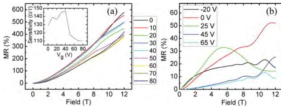
FIG. 2. (Color online) (a) MR for a typical shunted device showing a \sim 600\% change. The inset shows the sensitivity of the device. The slight oscillations are attributed to SdHO. (b) MR for a typical un-shunted device showing a much smaller change. The SdHO are much more pronounced.
