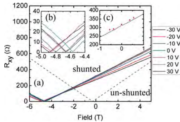
FIG. 3. (Color online) (a) R_{xy} vs. Field for various gate voltages for an externally shunted device. The black dashed line shows an un-shunted device. The minimum (intercept) moves further to the left for more chemically doped devices. (b) A close-up of the minimum. (c) A comparison of low temperature (4.2 K = black line) to room temperature (293 K = red points) data for resistance vs. field. There is a little resistance change.
