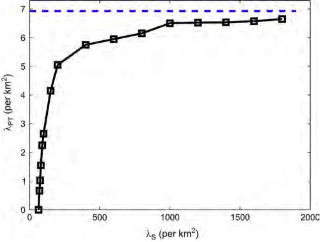
Fig. 6. Simulated connectivity regions when r_p = 150 m, r_I = 240 m, R_p = 100 m and R_I = 120 m. The blue dashed line is the upper bound (4) on the critical density \lambda_{PT}^* of primary transmitters given in T2.2. The area of the simulated heterogeneous network is 2000 \text{ m} \times 2000 \text{ m} . For a fixed density \lambda_S of the secondary users, the upper boundary \lambda_{PT}^*(\lambda_S) is equal to the minimum density of the primary transmitters such that over all the 1000 realizations, the percentage of the ones in which there exists at least one L-R crossing is below 50%. The intuitive reason for choosing the existence of an L-R crossing as the criterion for connectivity is illustrated in Fig. 5 and is discussed in Section V-C.
