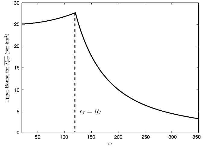
Fig. 9. Example of the upper bound on \bar{\lambda}_{PT}^* as a function of r_I (parameters are given by R_I = 120 \text{ m} , r_p = 0.625 r_I ).
