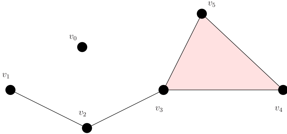
Fig. 4. A simplicial complex \Delta with 6 vertices (0-dimensional simplices: \{v_0\}, \{v_1\}, \{v_2\}, \{v_3\}, \{v_4\}, \{v_5\} ), 5 edges (1-dimensional simplices: \{v_1, v_2\}, \{v_2, v_3\}, \{v_3, v_4\}, \{v_3, v_5\}, \{v_4, v_5\} ), and 1 filled triangle (2-dimensional simplex: \{v_3, v_4, v_5\} ).
