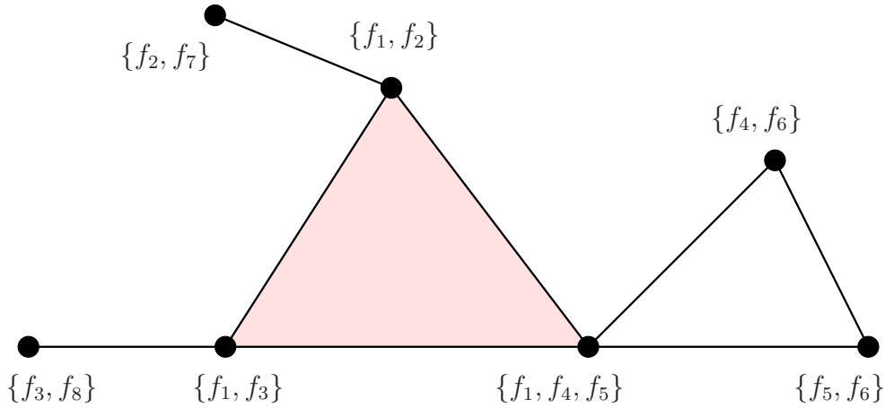
Fig. 2. An illustration of an MR-MC network and the constructed simplicial complex. The parameters within the braces are the channels which each node can access. In the communication graph derived from the network, a link exists between two nodes if and only if two nodes are within each other's transmission range and they share at least one common channel. Notice that a clique in the communication graph may not be a clique in the MR-MC network (correspondingly, a simplex in the simplicial complex), e.g., the three nodes of the right empty triangle.
