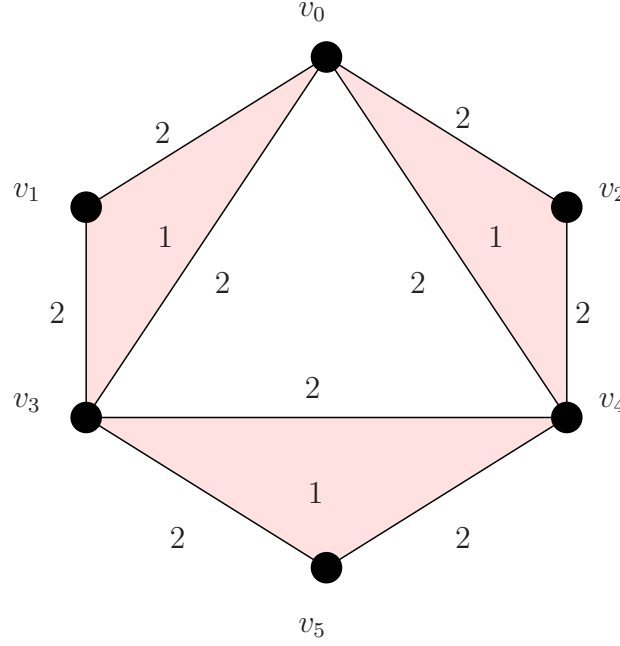
Fig. 3. A simplicial complex where its MCSSub is the three filled triangles, and is not a “tree” (the integers are the weights of the simplices).
