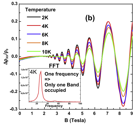
Fig. 2. (a) Shubnikov-de Haas oscillations seen in the sheet resistance at 2 K (sample A1). (b) The oscillatory behavior is plotted for various temperatures removing the parabolic dependence due to hole–hole interaction. The oscillations are periodic vs. 1/B , with a single frequency as verified from taking a fast Fourier transform on the data (inset b).
