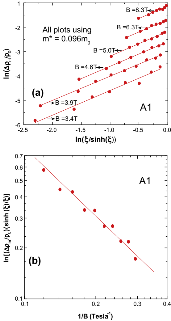
Fig. 3. (a) Effective hole mass is calculated using the temperature dependence of the oscillations as the value for which a gradient of unity is obtained in the plot of \ln(\frac{\Delta\rho}{\rho_0}) , vs. \ln(\frac{\xi}{\sinh \xi}) . (b) Dingle plot: Slope of line is -\pi\alpha/\mu where \alpha is the ratio \tau/\tau_q of the transport time \tau to the quantum lifetime \tau_q .
