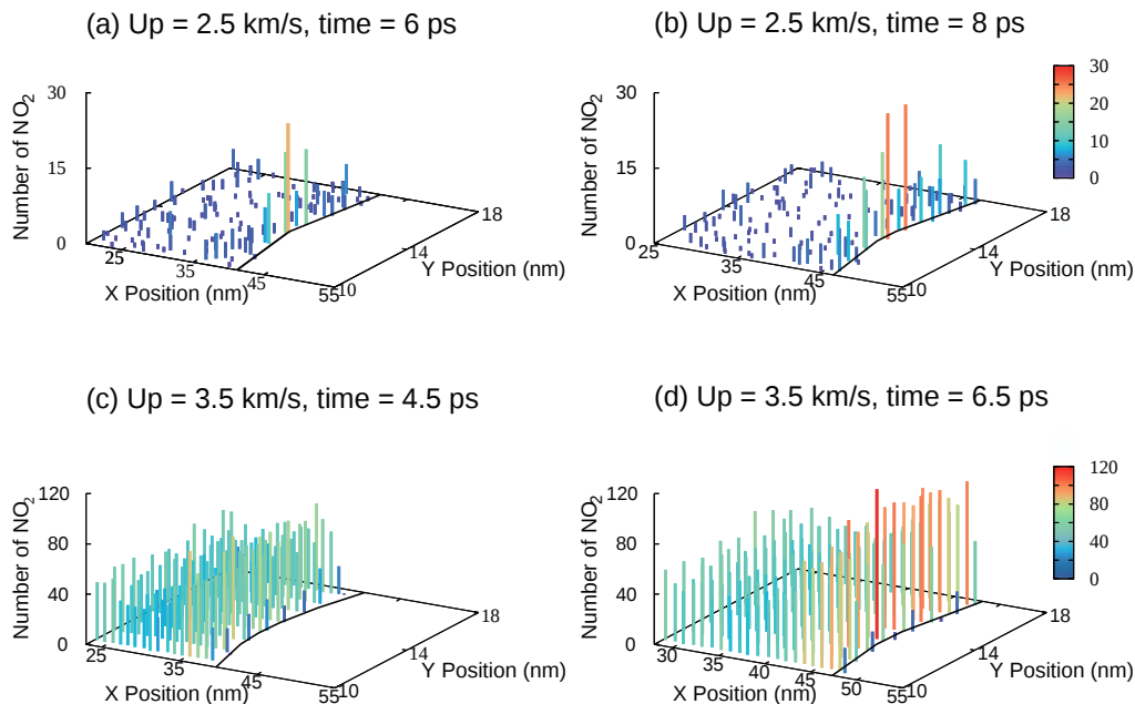
FIG. 3. (Color online) 2D distribution and time evolution of chemistry ( \text{NO}_2 formation) for various U_p . (a) U_p = 2.5 km/s at t = 6.0 ps: The chemical reaction has occurred mainly in the hot-spot region. (b) U_p = 2.5 km/s at t = 8.0 ps: Additional chemical reactions have occurred and a small amount of \text{NO}_2 has diffused to the polymer region (the right region of the solid line in the xy plane). (c) U_p = 3.5 km/s at t = 4.5 ps: The chemical reaction occurs in the shocked regions but much more occur in the hot-spot region. (d) U_p = 3.5 km/s at t = 6.5 ps: We see diffusion of \text{NO}_2 into the polymer region.
