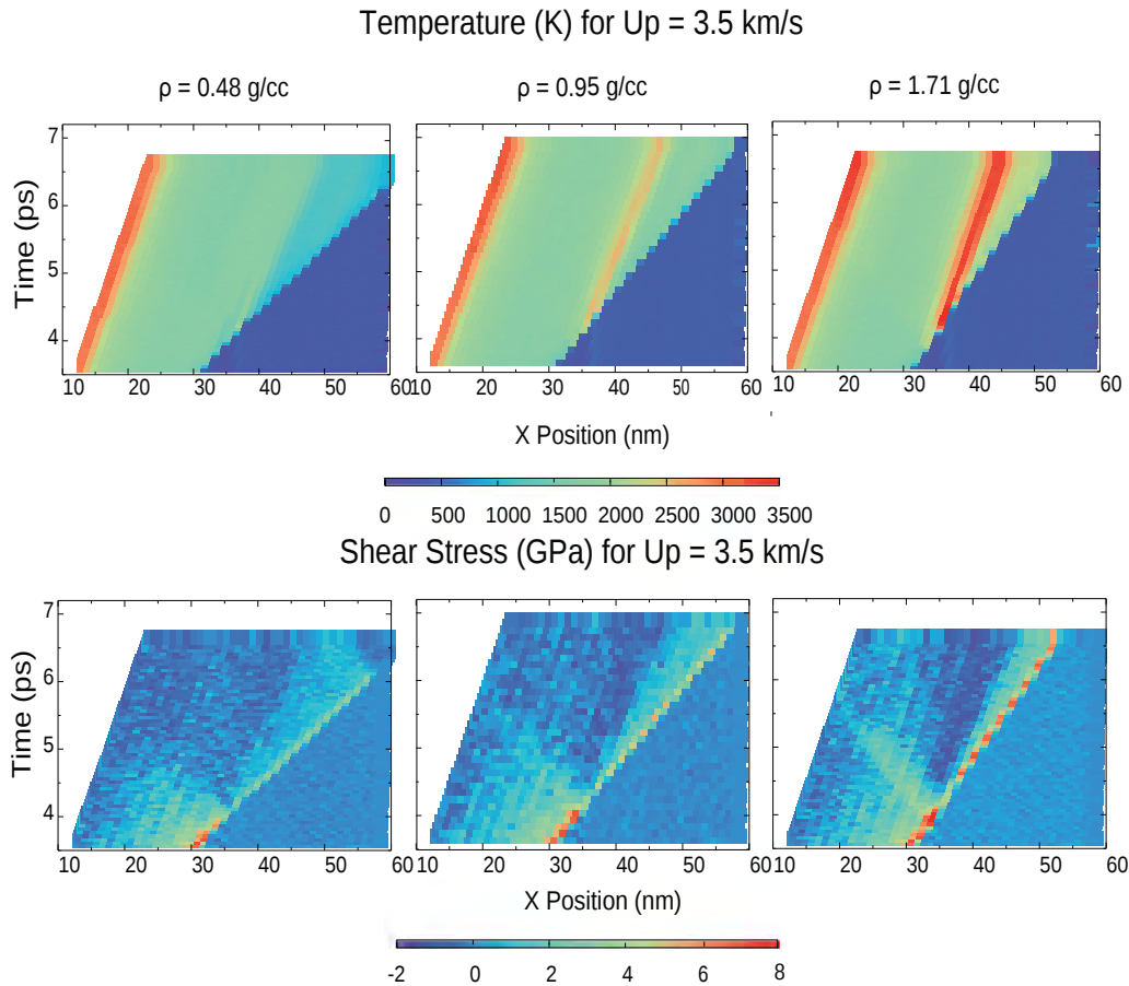
FIG. 4. (Color online) The dependence of hot-spot formation (temperature and shear stress) on the density of the polymer binder at a shock velocity of 3.5 km/s. The middle ( 0.95 \text{ g/cm}^3 ) is normal density. Thus using of a polymer with half the normal density prevents hot-spot formation. This is due to the improved interface impedance which allows reflective rarefaction wave relaxation. In contrast, increasing the binder density enhances the hot spot due to the reflective shock waves reflected back into the RDX.
