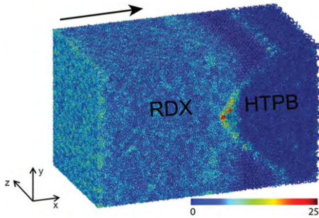
FIG. 1. (Color online) Snapshot of PBX during shock loading at U_p = 2.5 km/s (for 6.0 ps). The shading is based on the total slip in angstroms. This system is 54 nm thick in the shock direction ( x ), with a period of 27 nm along the sawtooth direction ( y ), and is uniform with a periodic length of 25 nm in the z direction. The arrow indicates shock direction.
