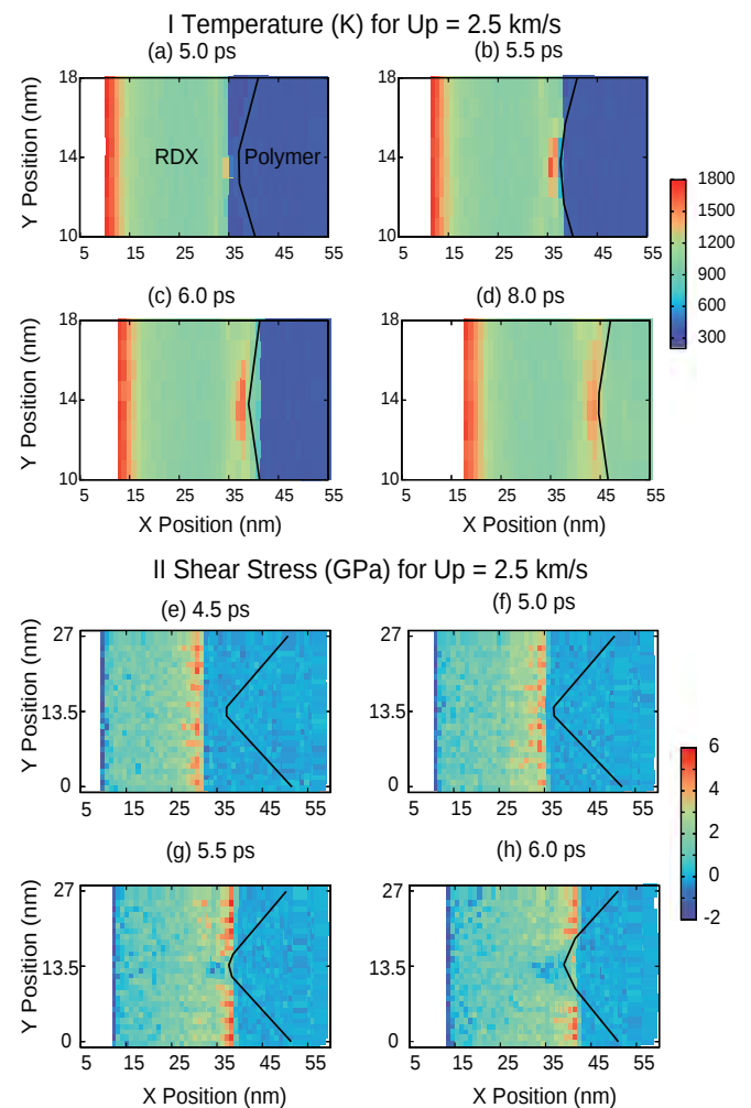
FIG. 2. (Color online) Time evolution of temperature and von Mises shear stress for U_p = 2.5 km/s at various stages during the shock compression. The solid line represents the interface position between the RDX and the binder. Shock wave propagates from left (RDX) to right (binder). (e) 4.5 ps, shock wave has not propagated to polymer; (a),(f) 5.0 ps, shock wave just reaches the interface; (b),(g) 5.5 ps, adiabatic shear localization in a small triangle interface region; (c),(h) 6.0 ps, shock wave has passed through the hot-spot region; (d) 8.0 ps, shock wave has passed through the interface.
