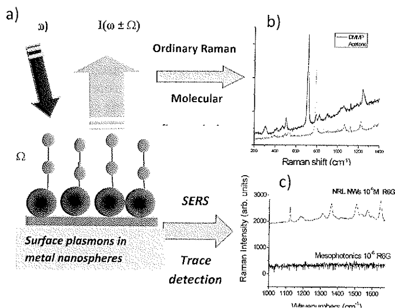
Figure 1. Raman scattering for liquids of acetone and DMMP (top right) and Surface enhanced Raman scattering for Rh6G (bottom right) using NRL dielectric NWs and commercial Mesophotonics substrates. The cartoon on the left shows the SERS effect.
