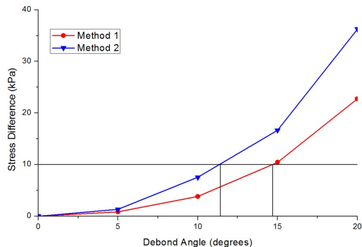
Fig. 10 -- A comparison of flaw detectability using two different methods of detection
