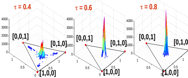
Fig. 4. Phase transition (top) of a society from radicalized beliefs to a consistent belief. Histogram (bottom) of 300 asymptotic opinion profiles with n = 100 at \tau = 0.4, 0.6, 0.8 .
