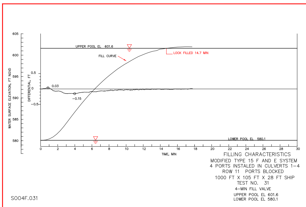
Figure 32. Time histories of water-surface and water-surface differential for 4-min filling valve operation with modified Type 15 Design (4 ports added in culverts 1-4 and row 11 ports blocked).
