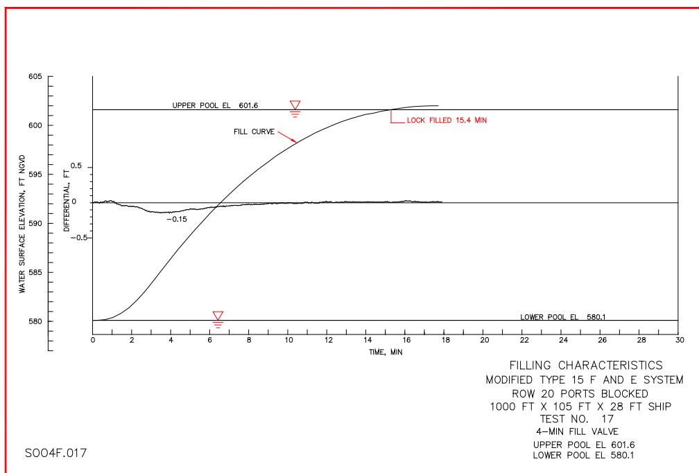
Figure 29. Time histories of water-surface and water-surface differential for a 4-min filling valve with Type 15 Chamber Design and row 20 ports blocked.
