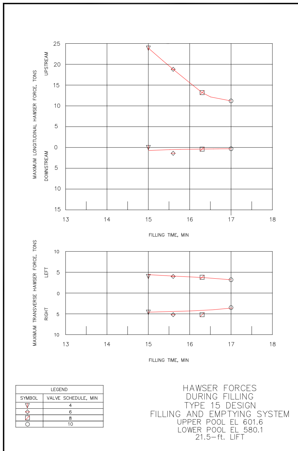
Figure 25. Average maximum hawser forces with Type 15 Chamber Design.
