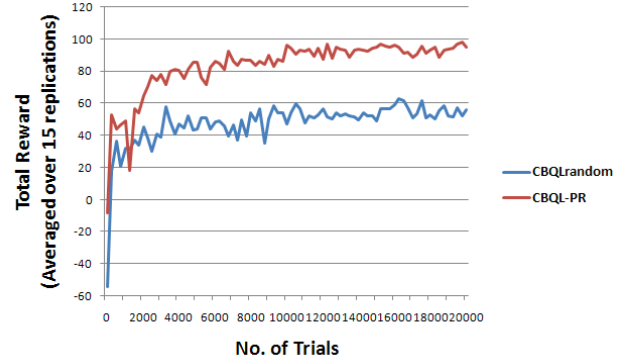
Figure 4: When using the same arity for the state representation, randomly predicting the defensive play performs poorly vs. using plan recognition’s predictions.
