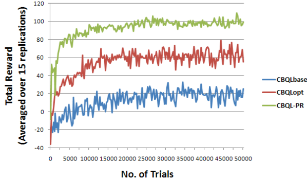
Figure 3: Comparison highlighting the utility of our plan recognition approach for a case-based reinforcement learner on the task of controlling the Rush 2008 QB’s actions.
