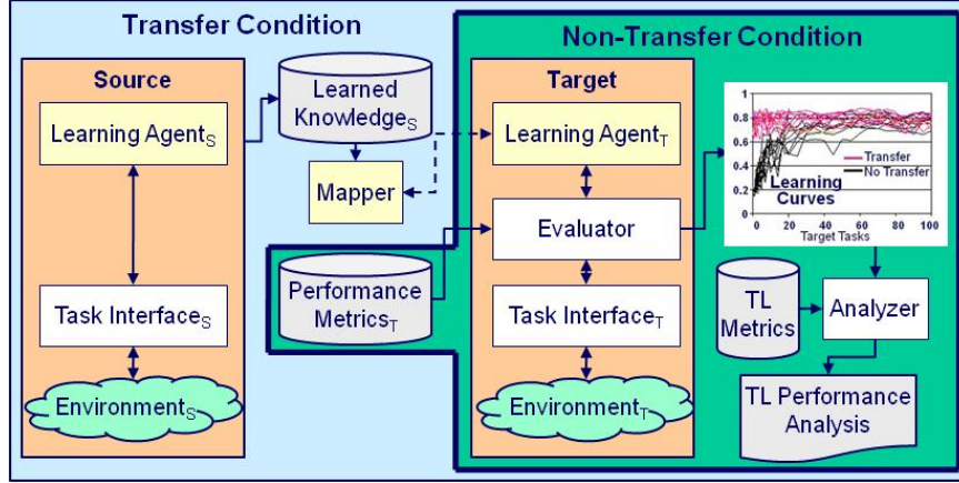
Figure 1: Transfer learning conditions, method, and evaluation strategy.
