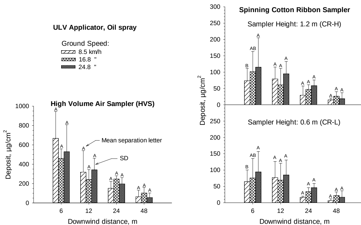
Figure 3 Oil-soluble tracer collected by high volume air samplers and spinning cotton ribbons at different travel speeds of the ULV applicator. Within each plot/downwind location, different mean separation letters indicate significant effect at the 5% level.
