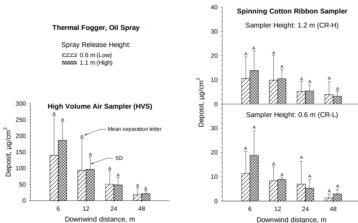
Figure 6 Oil-soluble tracer collected by high volume air samplers and spinning cotton ribbons at two release heights of the thermal fogger. Within each plot/downwind location, different mean separation letters indicate significant effect at the 5% level.
