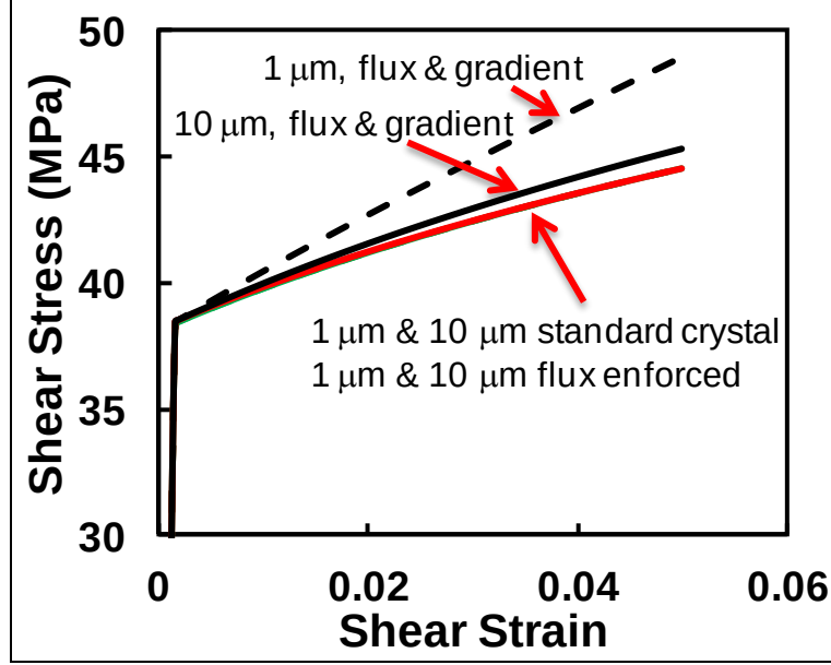
Figure 11. Stress strain curves from 1- \mu m-thick and 10- \mu m-thick films with standard crystal plasticity, with dislocation flux enforced and with flux enforced plus gradient strengthening.
