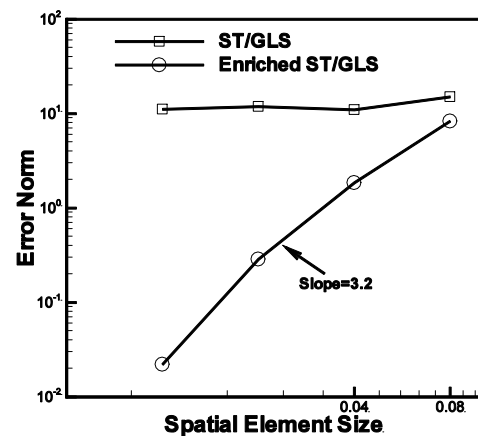
Figure Qia-3: Error norm vs. spatial element size between regular and enriched space-time solutions.
