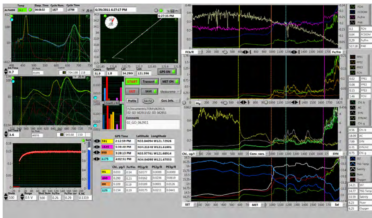
Fig. 8. A transect map and a screenshot of the ALFA operational software taken during the underway frontal study with the ALFA instrument in the California Current System, CCE LTER cruise, June 2011. Right panels display spatial distributions of Chl a (green), CDOM (dark-blue, upper panel), Fv/Fm (magenta), PAR (beige), PBP pigments (yellow-orange), temperature (blue), salinity (white), and oxygen (red).
