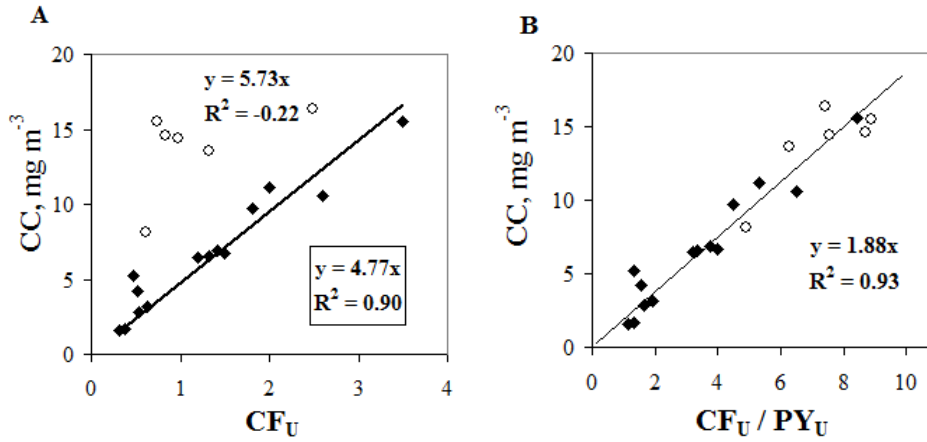
Fig. 4. (A) Correlation between measurements of Chl concentration (CC) in water samples and underway Chl fluorescence measurements at the sampling locations (CF U ). Black dots and empty circles represent the data from the dark-time and morning portions of the transect, respectively. The framed and unframed regression equations are calculated for the dark-time and entire data sets, respectively. (B): Correlations between CC in water samples and fluorescence parameter CF/PY calculated from Chl fluorescence (CF) and PSII photochemical yield (PY) underway flow-through measurements (the same data set as in panel A).
