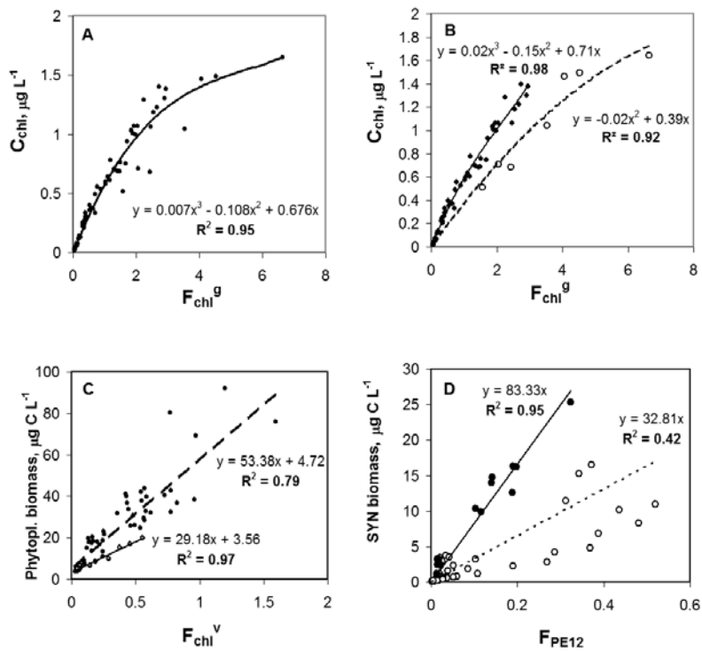
Fig. 5. (A): Correlation between chlorophyll a (Chl a) concentration ( C_{chl} ) and Chl a fluorescence ( F_{chl} ) measured with ALF instrument. (B): Same data as in panel A; a subset of samples from the diatom-dominated Chl a maximum at the front is displayed with empty circles. (C): dashed regression line – correlation between autotrophic carbon biomass (AC) and Chl a fluorescence ( F_{chl} ) measured with ALF instrument; solid regression line – correlation for a subset of samples collected between 40 m and 80 m at Stns. 1-3. (D): dashed regression line - correlation between phycoerythrin fluorescence of Synechococcus ( F_{PE12} ) and their carbon biomass (SYN); solid regression line - correlation for a subset of the samples (filled dots) collected in the subsurface layer above the Chl a maximum.
