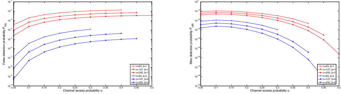
(a) False detection probability v.s. channel access probability (b) Miss-detection probability v.s. channel access probability
